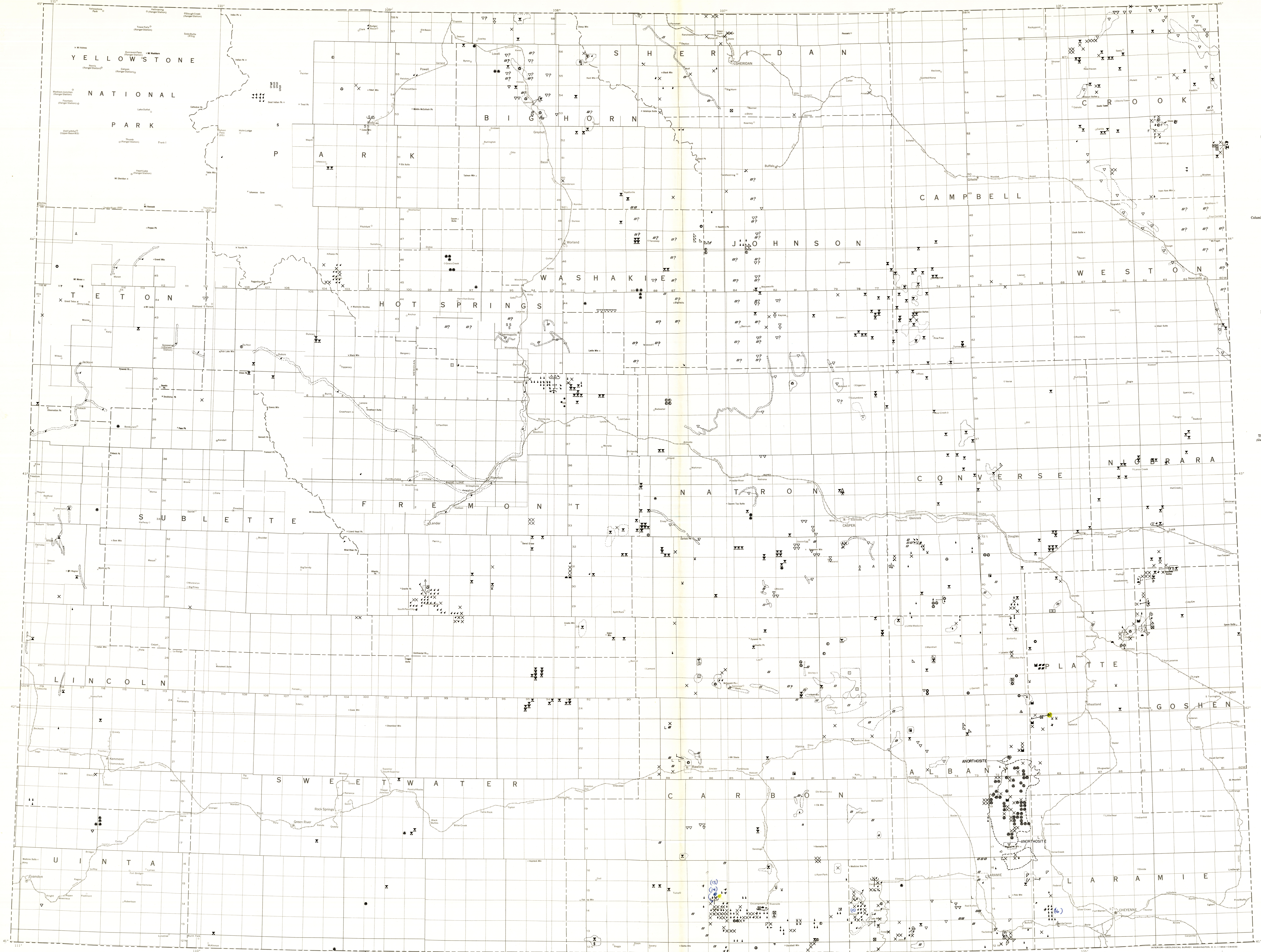
REPORTED OCCURRENCES OF SELECTED MINERALS IN WYOMING Includes most metals and nonmetals; does not include mineral fuels, sodium and potassium salts, or phosphate
