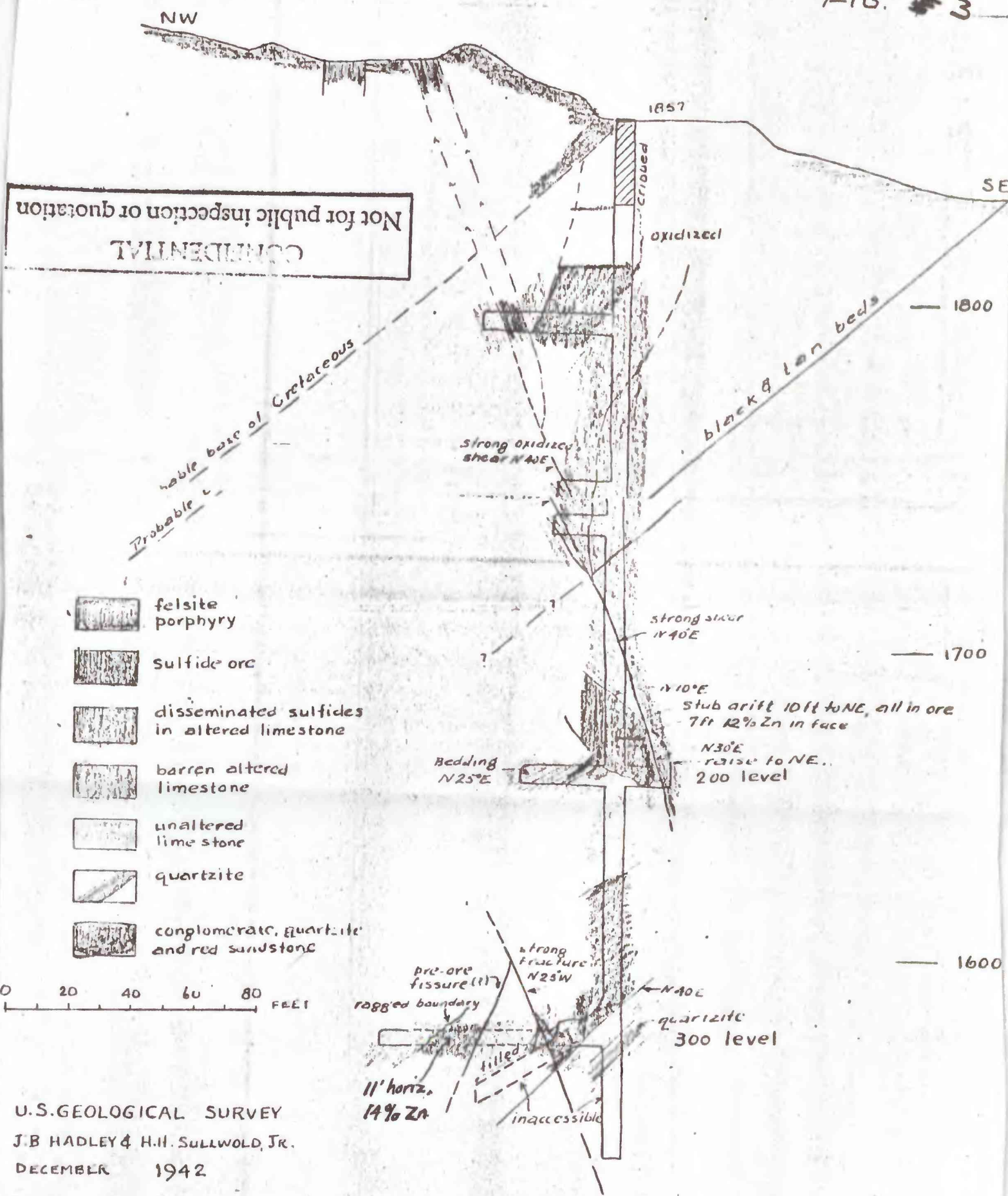
NW-SE SECTION AT PHONODOREE SHAFT REWARD DISTRICT, PINAL CO., ARIZ.
