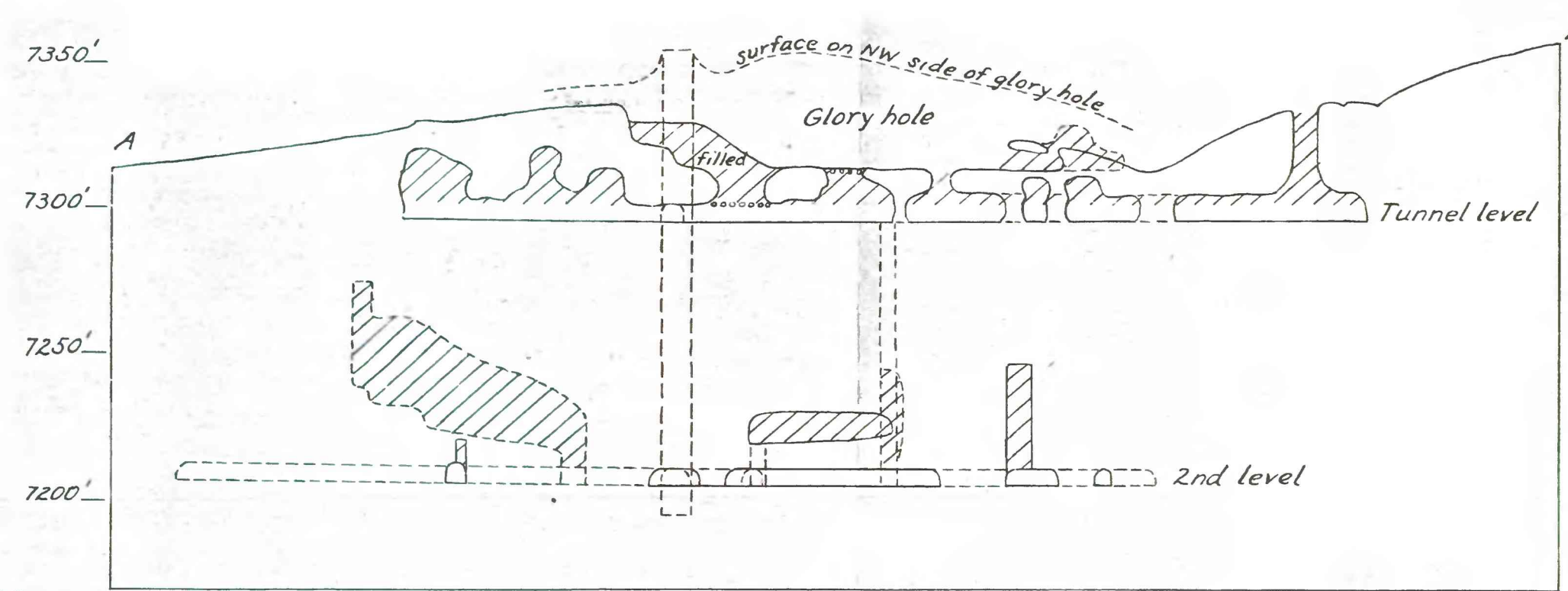
LONGITUDINAL PROJECTION ON SECTION A-A', SHOWING STOPE
