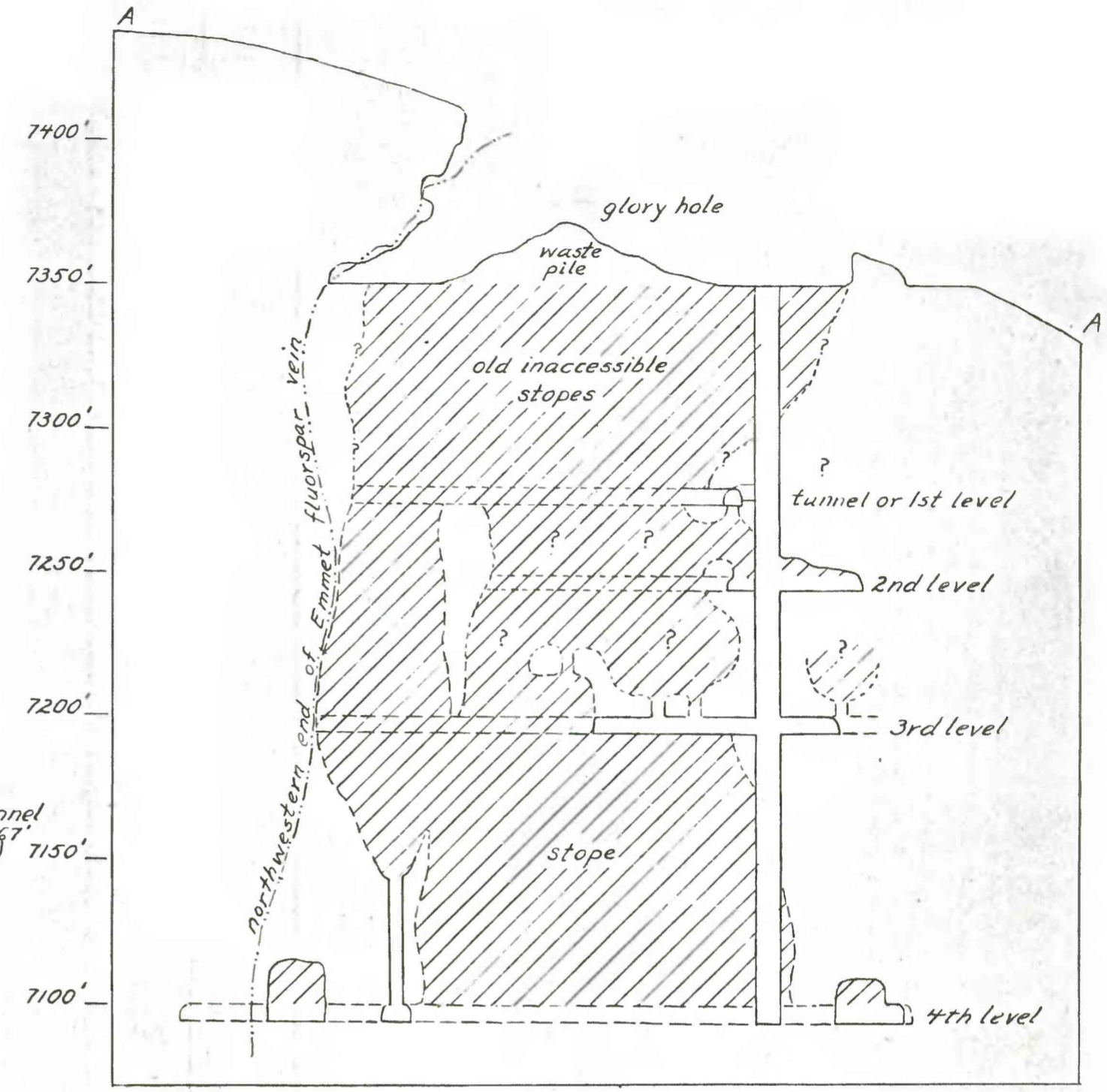
LONGITUDINAL PROJECTION ON SECTION A-A' SHOWING STOPES
