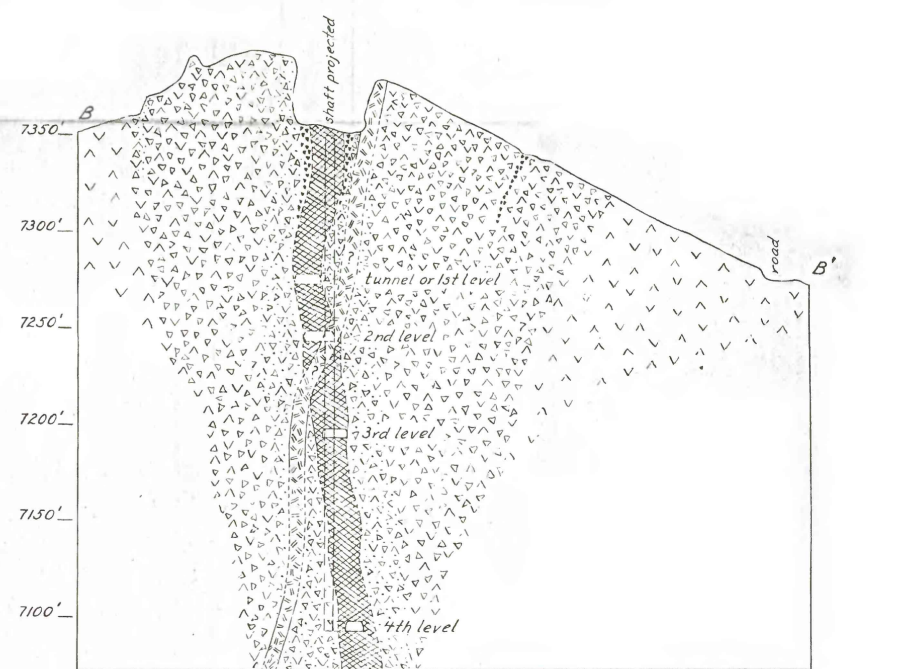
SECTION B-B' SHOWING GENERAL SHAPE OF VEIN (Outline of stopes omitted because of lack of sufficient data)
