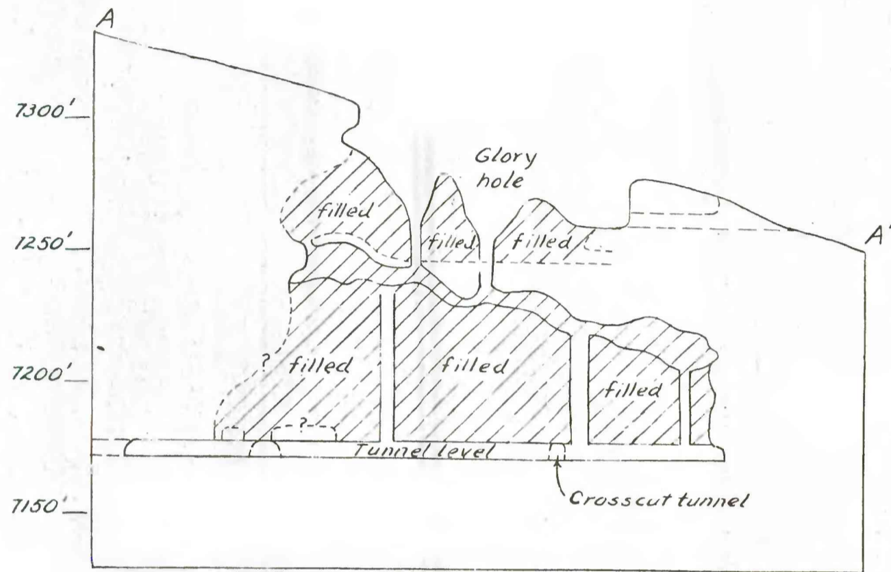
LONGITUDINAL PROJECTION ON SECTION A-A', SHOWING SLOPES
