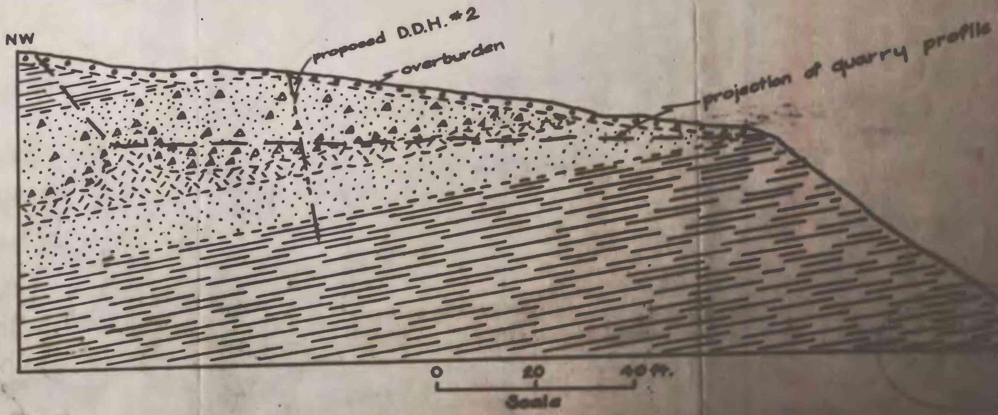
Fig. 1 Cross-section A-A; Arlington Copper Mine. Explanation same as Plate 1. Intensity apparently most intense immediately above trap.
