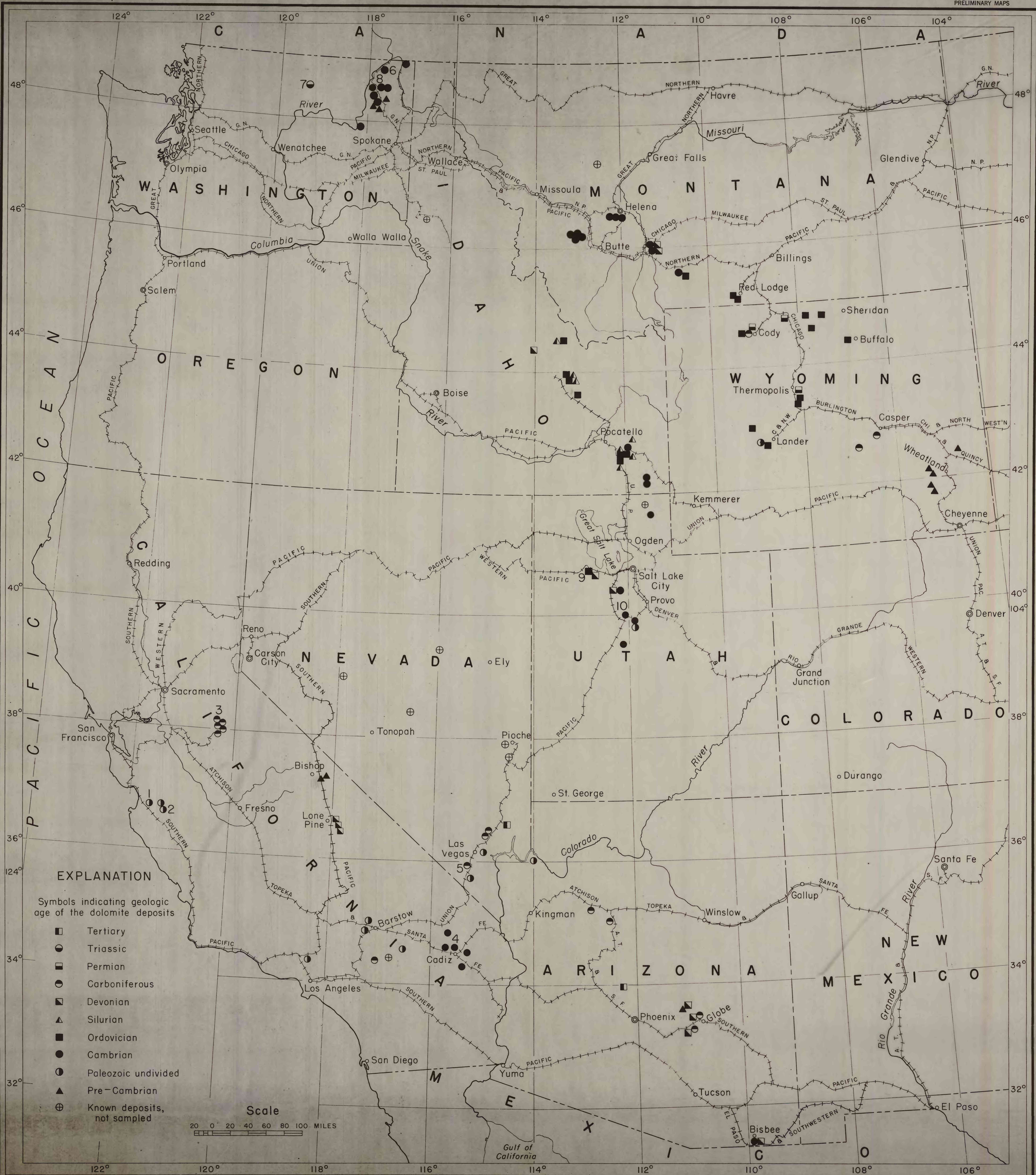
INDEX MAP OF WESTERN UNITED STATES SHOWING DISTRIBUTION AND AGE OF DOLOMITE DEPOSITS
