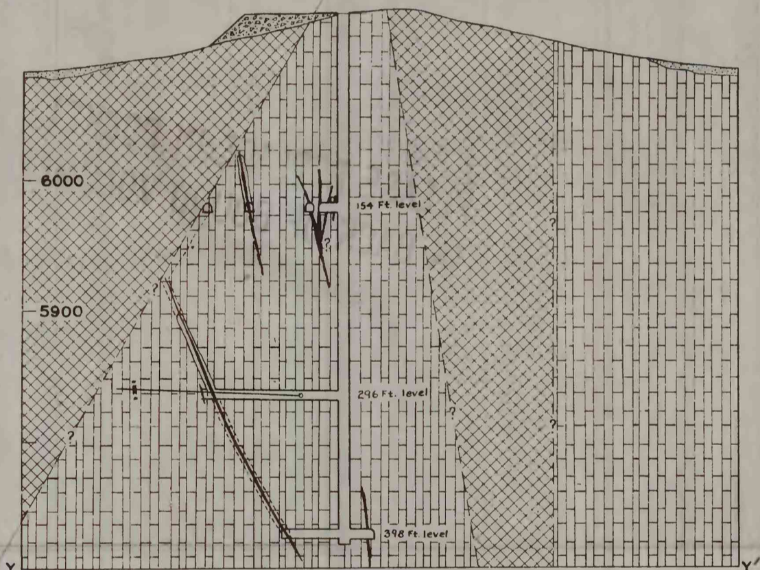
SECTION ALONG LINE Y-Y'
