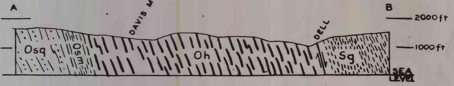
GEOLOGIC SECTION ALONG LINE A-B
