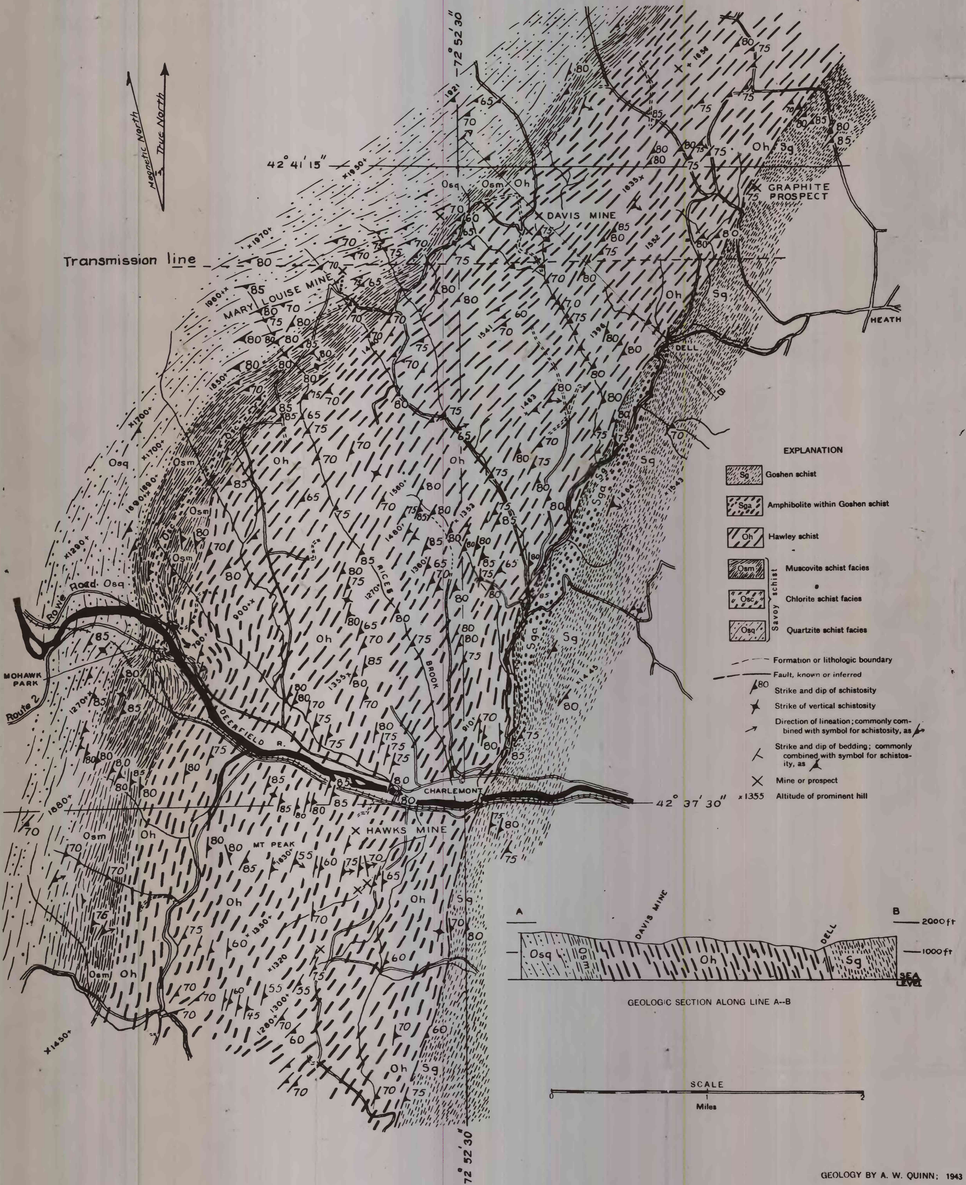
PLATE 1. BEDROCK GEOLOGIC MAP OF THE CHARLEMONT-HEATH AREA, MASS.
