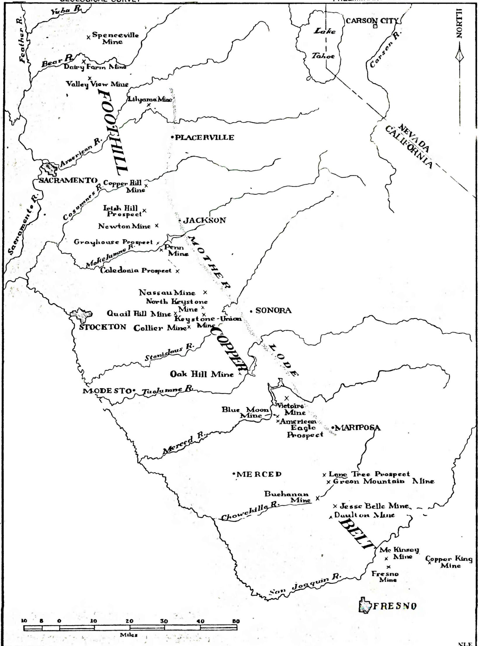
INDEX MAP, FOOTHILL COPPER BELT, CALIFORNIA
