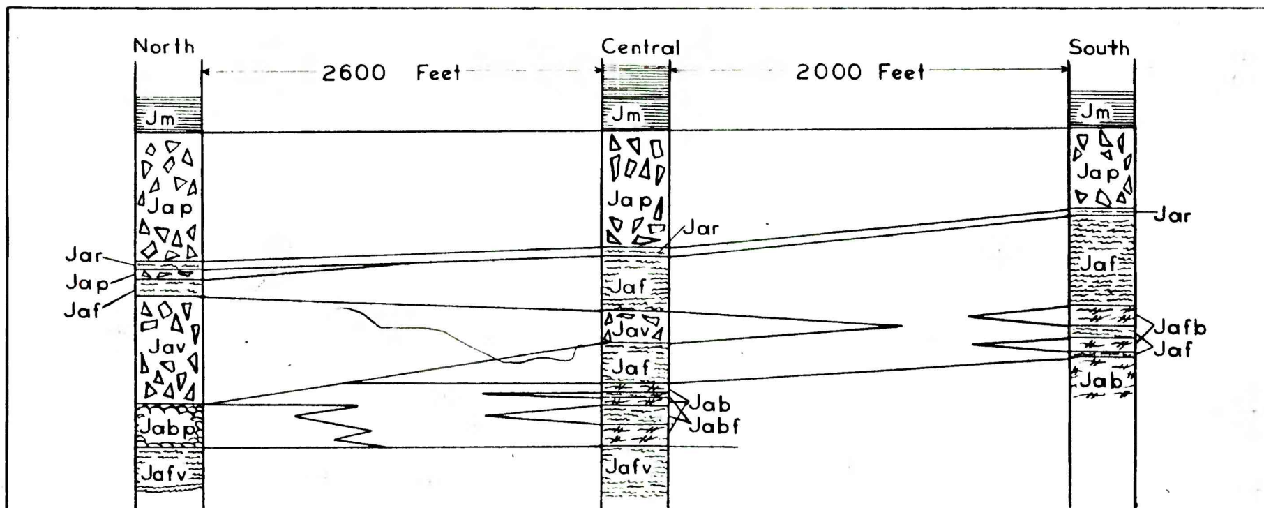
Columnar sections of stratigraphic units at the PENN MINE Calaveras County, California
