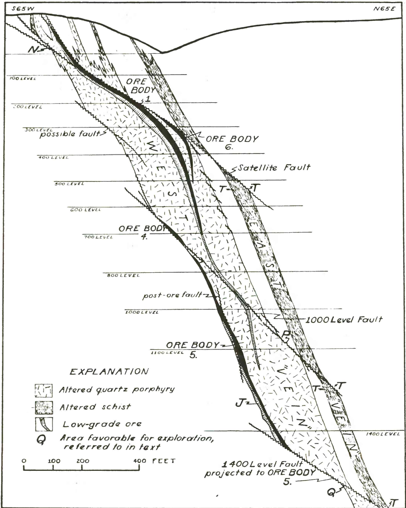
Composite Section through the No.2 Shaft Area, PENN MINE Calaveras County, California.
