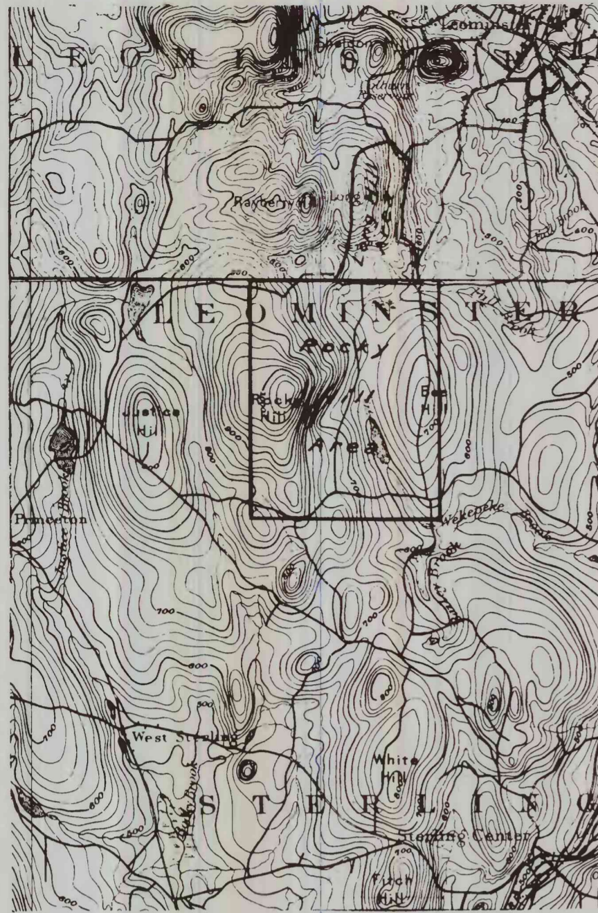
FIGURE 1.— KEY MAP, TO SHOW LOCATIONS OF ROCKY HILL AND LONG HILL PEGMATITE AREAS. [PARTS OF FITCHBURG AND WORCESTER MASSACHUSETTS QUADRANGLES]
