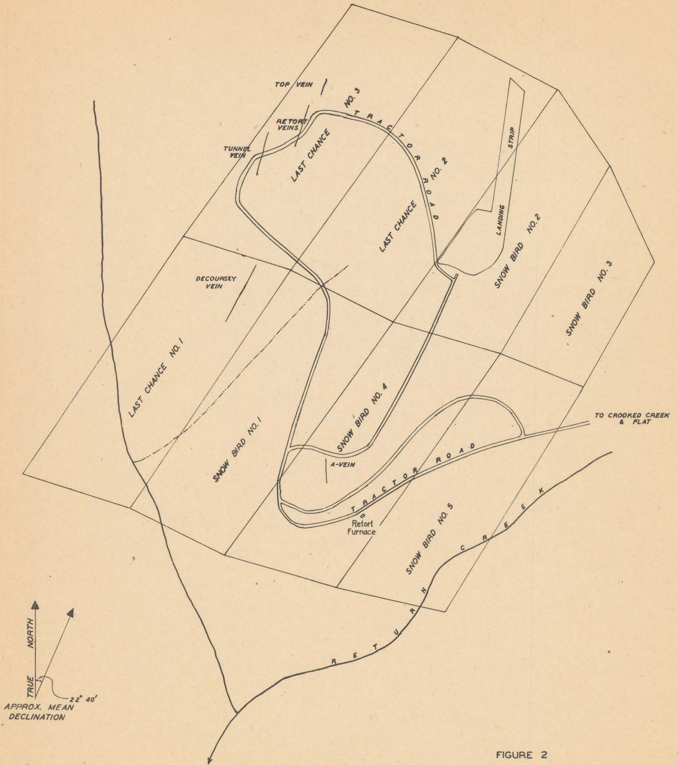
FIGURE 2 MAP SHOWING LODE MINING CLAIMS DECOURSEY MOUNTAIN AREA QUICKSILVER DEPOSITS IDITAROD DISTRICT, SOUTHWESTERN ALASKA
