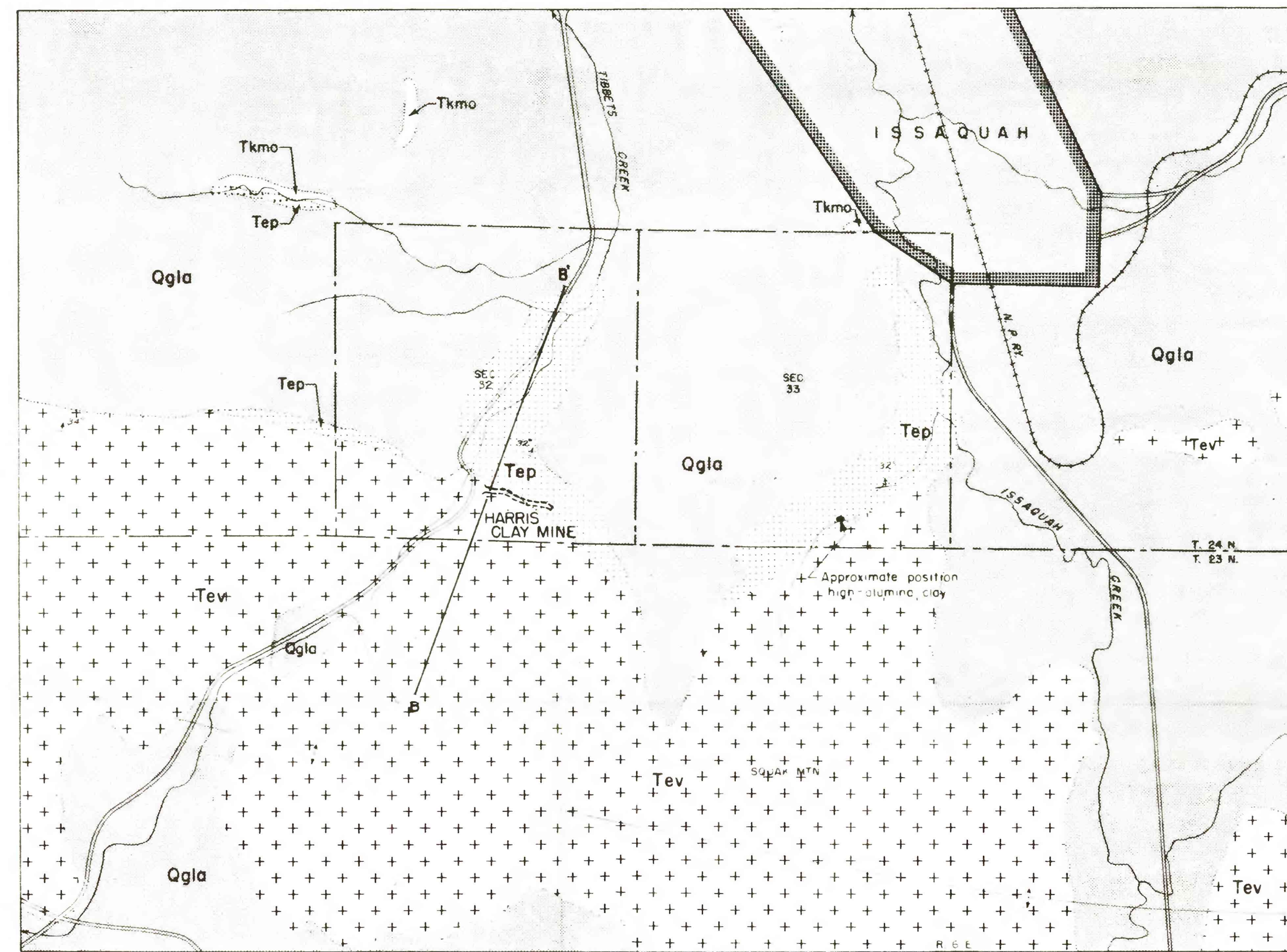
GEOLOGIC MAP
