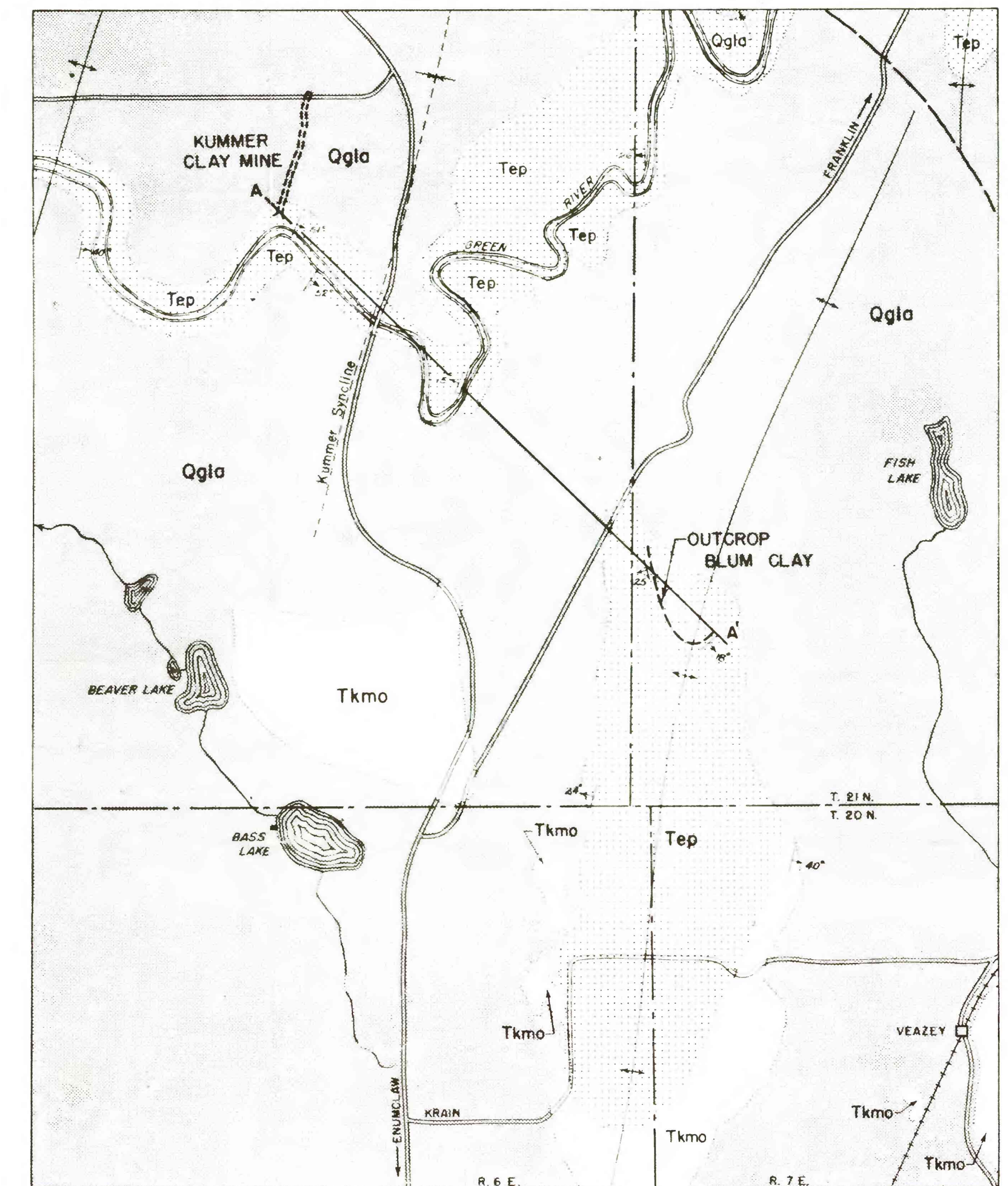
GEOLOGIC MAP
