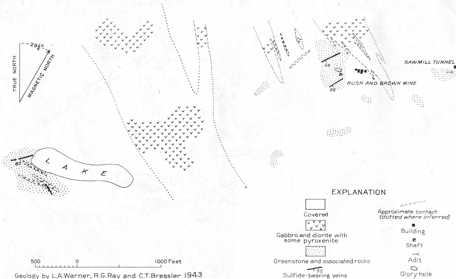
GENERALIZED GEOLOGIC MAP OF THE RUSH AND BROWN MINE AREA KASAAN PENINSULA, PRINCE OF WALES ISLAND, SOUTHEASTERN ALASKA
