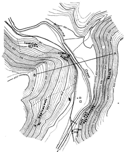
DAM SITE
