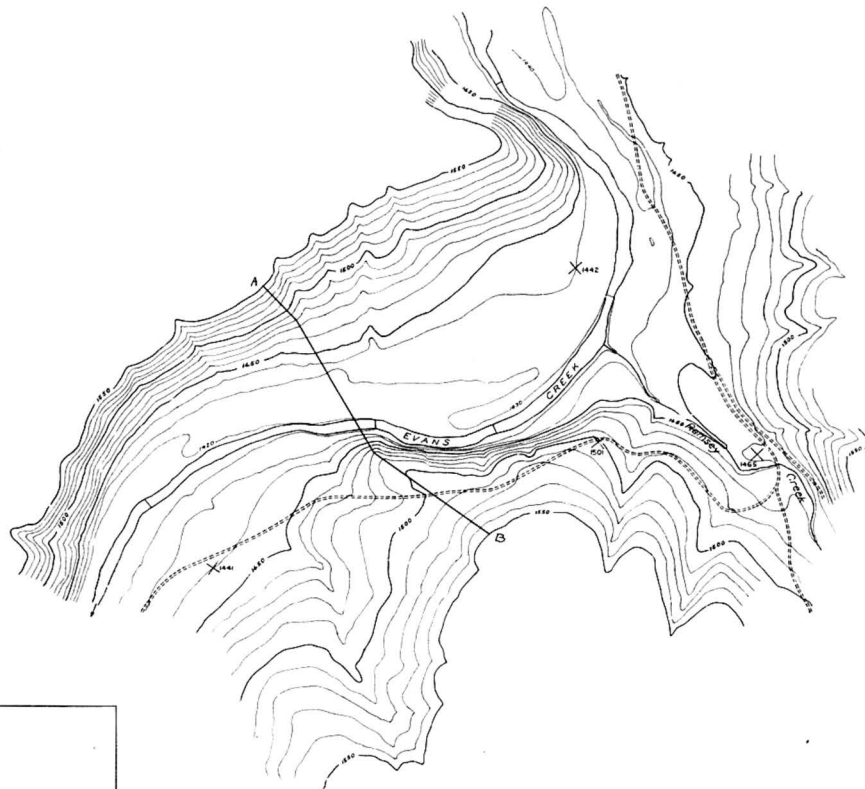
Fig. 5 UPPER EVANS CREEK DAM SITE
