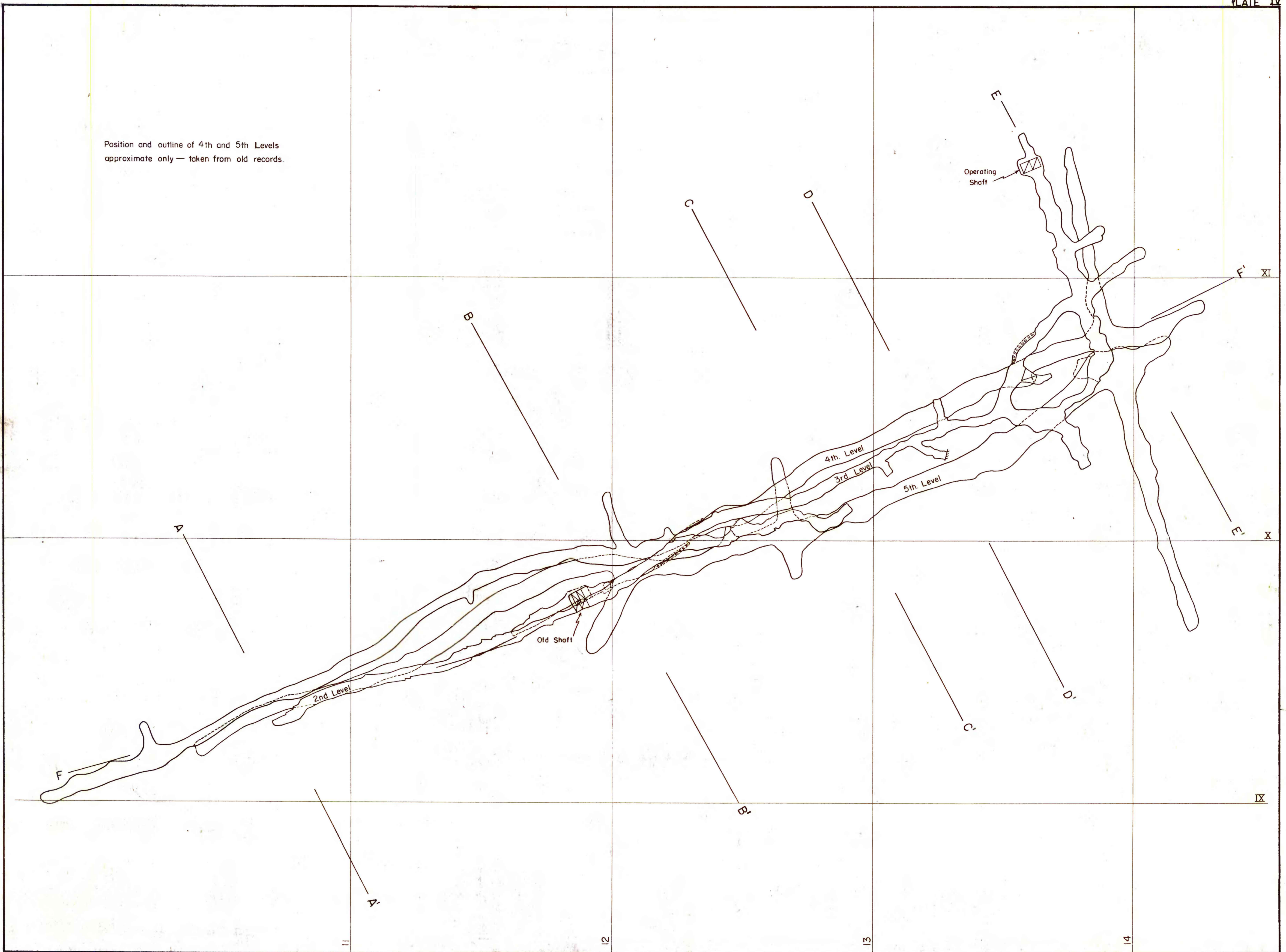
COMPOSITE MAP OF UNDERGROUND WORKINGS, CARISSA MINE, FREMONT COUNTY, WYOMING
