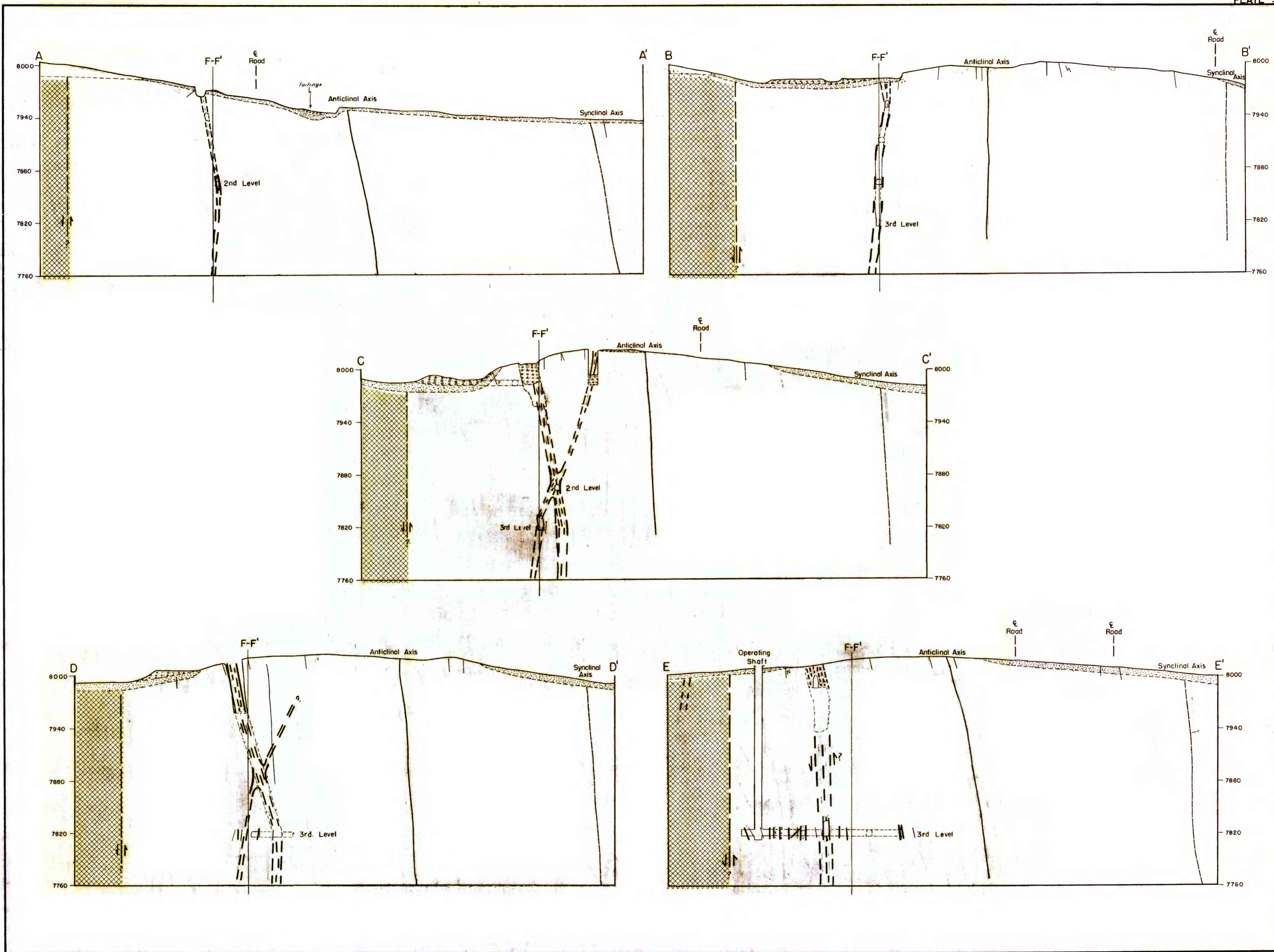
CROSS SECTIONS, CARISSA MINE, FREMONT COUNTY, WYOMING
