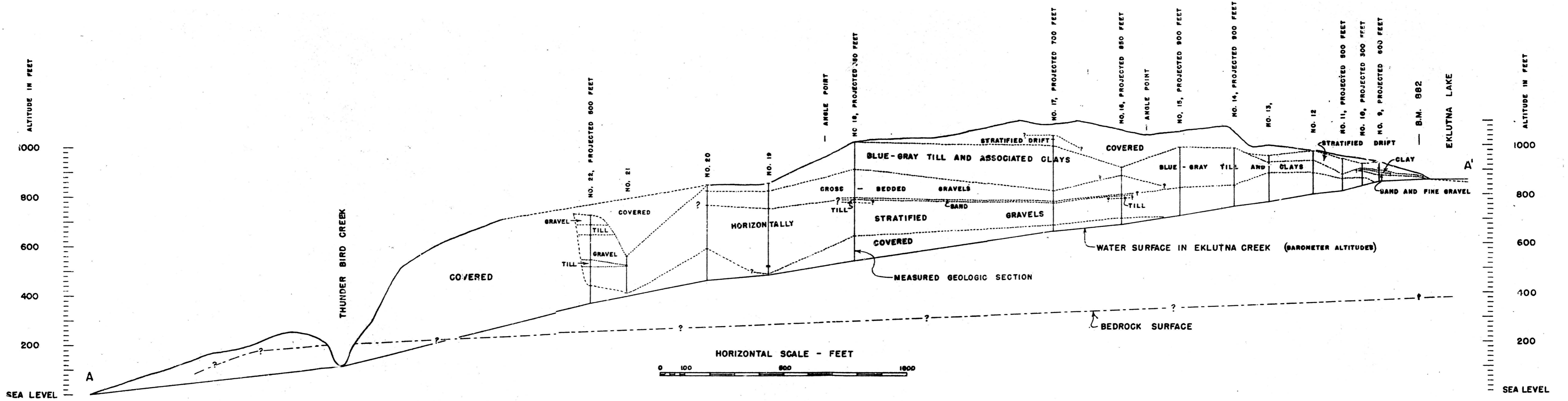
GEOLOGIC PROFILE OF EKLUTNA VALLEY ALONG LINE A-A'
