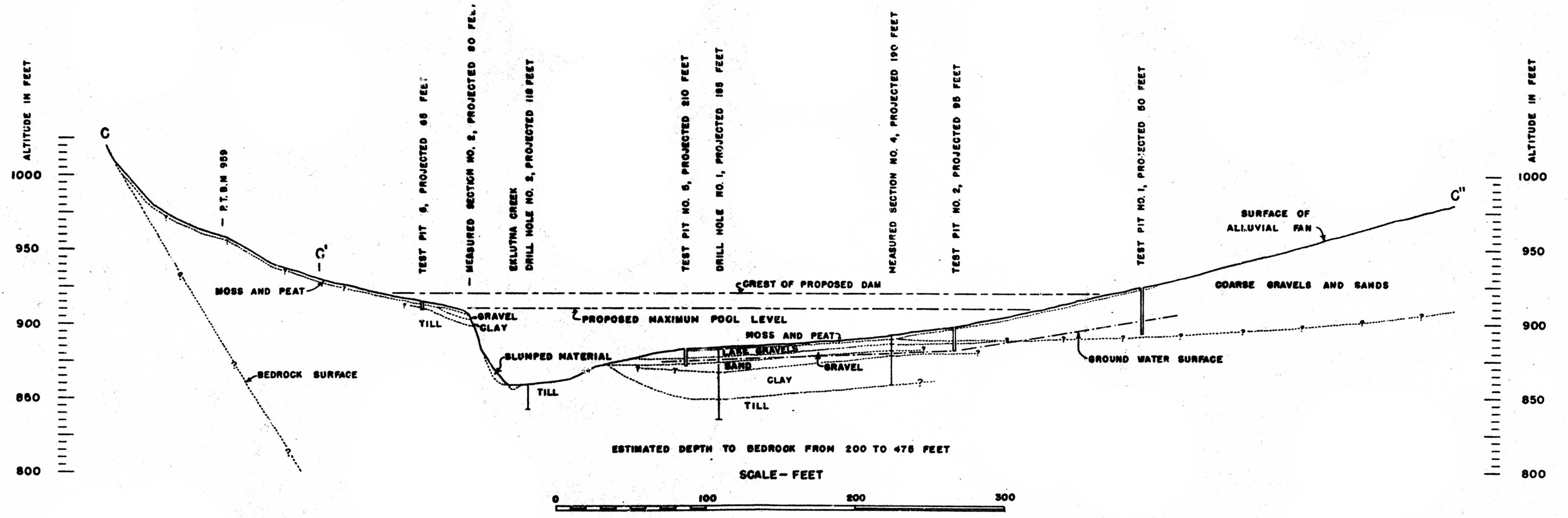
GEOLOGIC CROSS SECTION ALONG AXIS OF PROPOSED DAM
