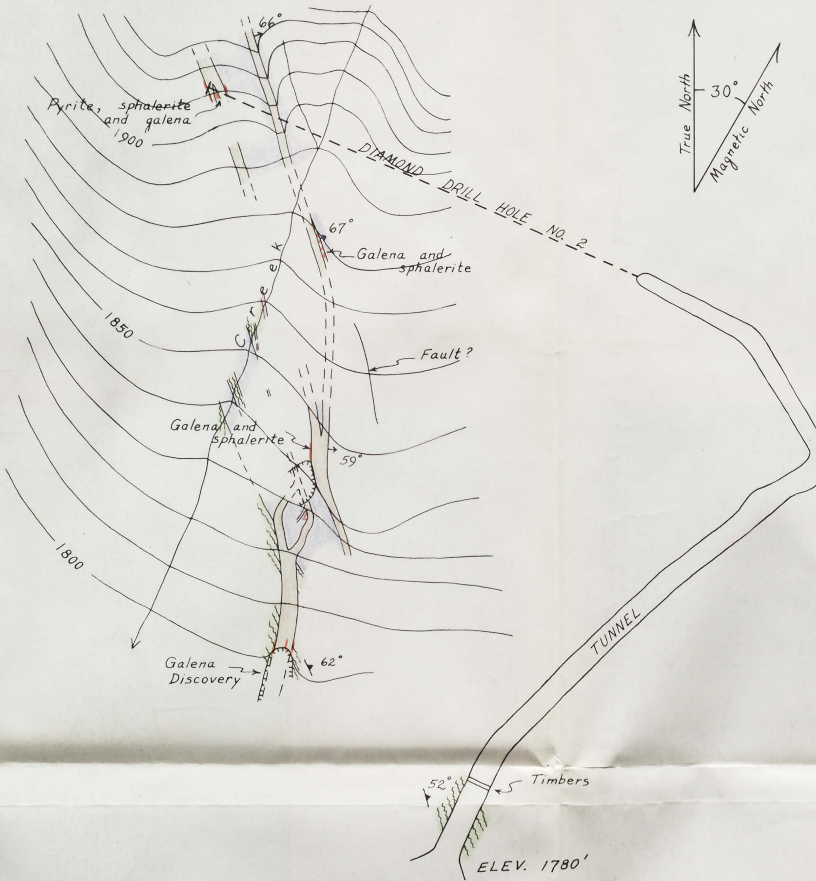
SKETCH MAP SHOWING RELATION OF SURFACE GEOLOGY TO DIAMOND DRILL HOLE NO. 2, BERG PROSPECT, SOUTHEASTERN ALASKA
