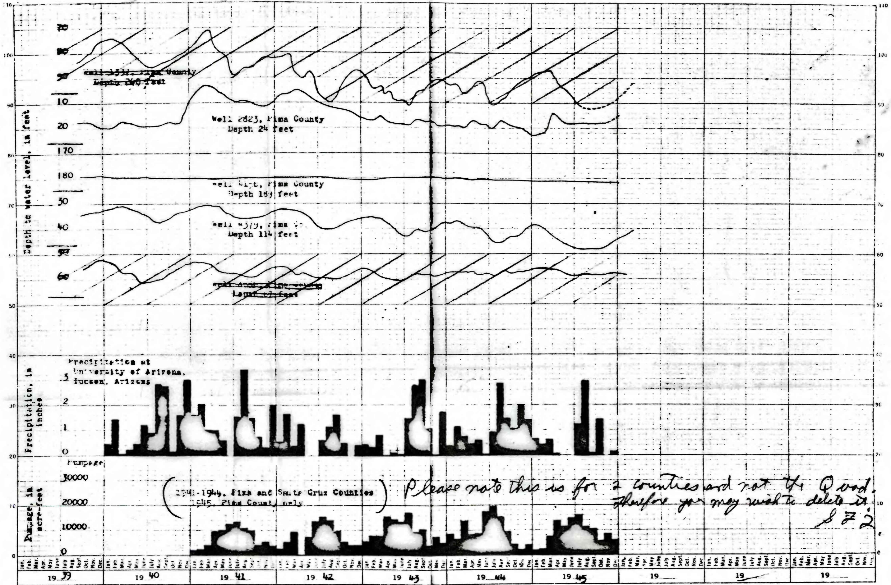
Figure - Graphs show fluctuations of water level in observation wells in the Santa Cruz Valley, Pima County, Arizona
