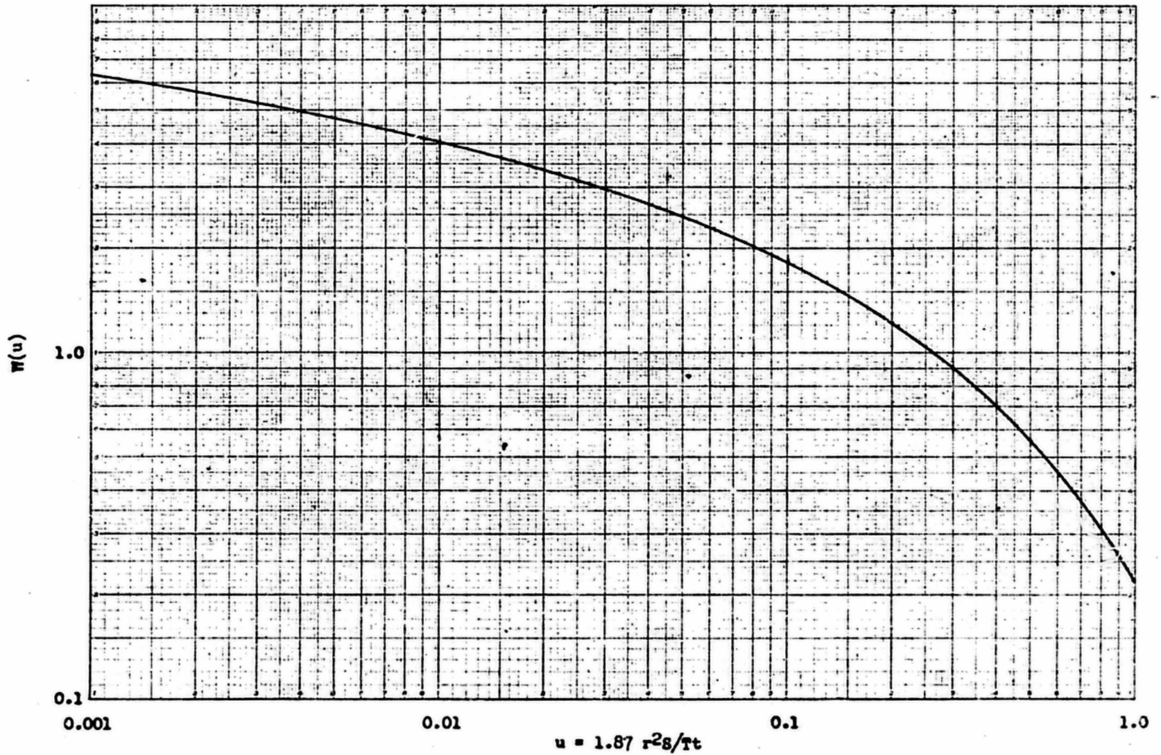
Fig. 12 -- Logarithmic graph of the exponential-integral "type curve"
