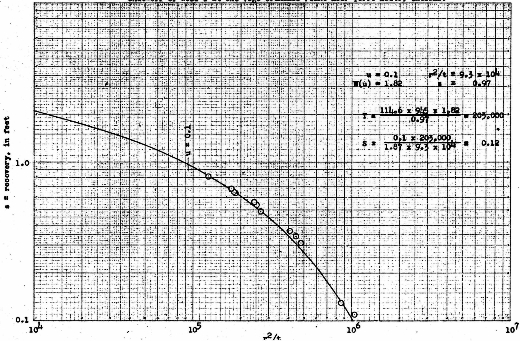
Fig. 13 -- Logarithmic graph of the recovery of water level in observation well P 2 after the shut-off of well 1 at the Vigo Ordnance Plant near Terre Haute, Indiana.
