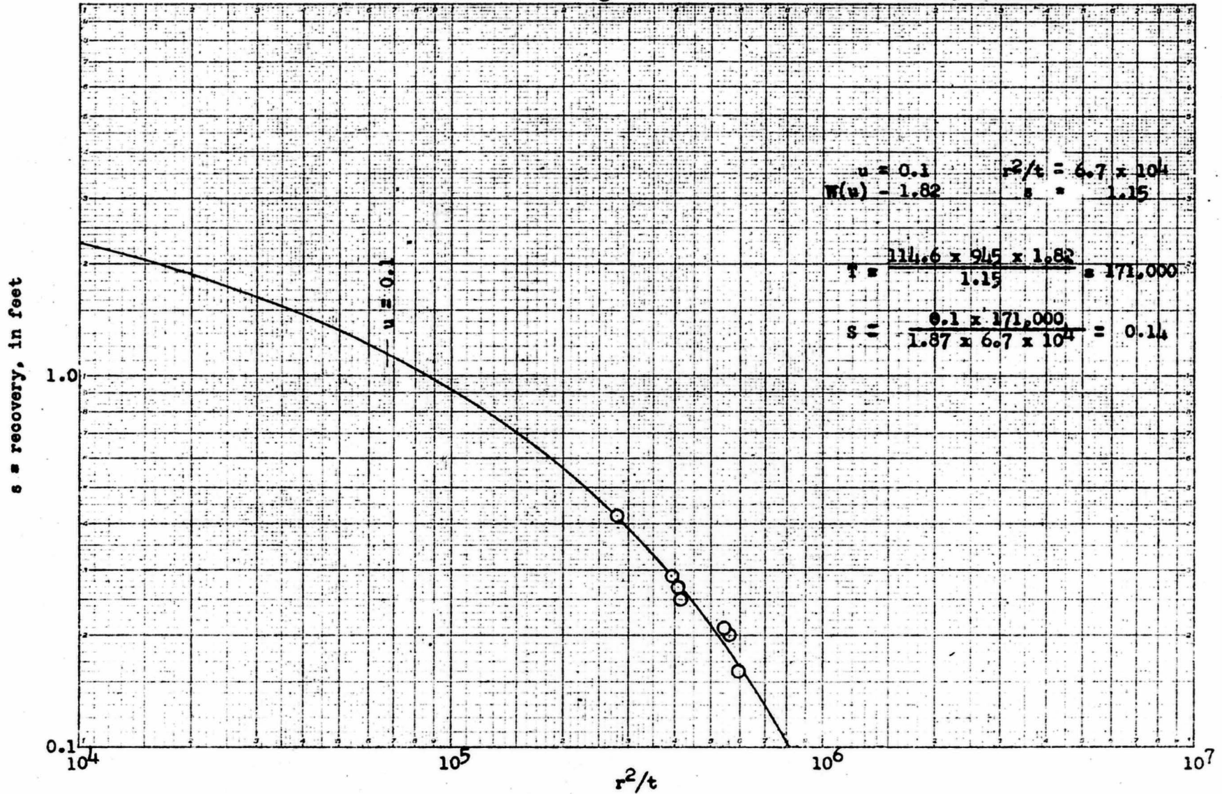
Fig. 14 -- Logarithmic graph of the recovery of water level in observation well P 3 after the shut-off of well 1 at the Vigo Ordnance Plant near Terre Haute, Indiana.
