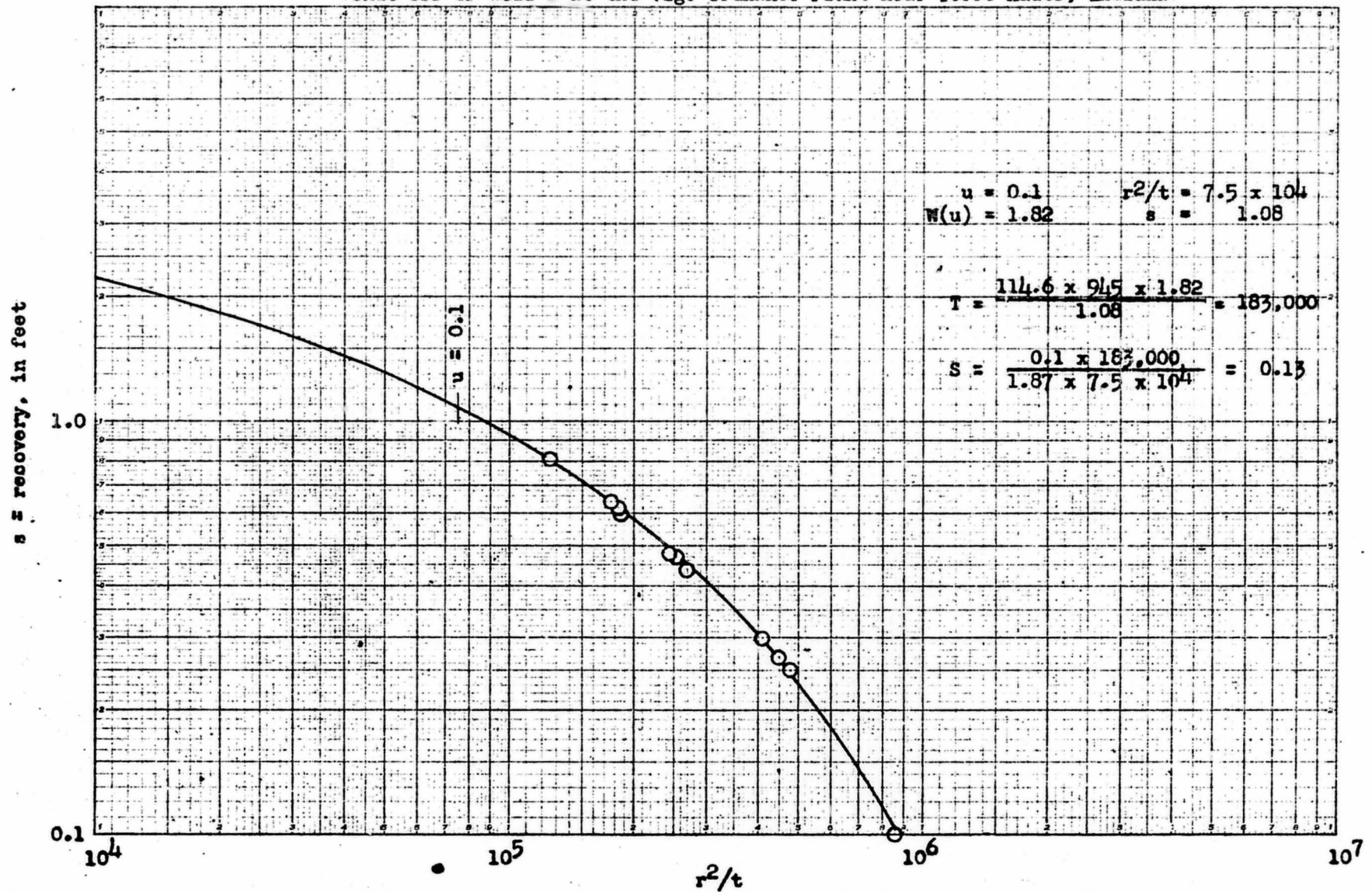
Fig. 15 -- Logarithmic graph of the recovery of water level in observation well P 3,1 after the shut-off of well 1 at the Vigo Ordnance Plant near Terre Haute, Indiana.
