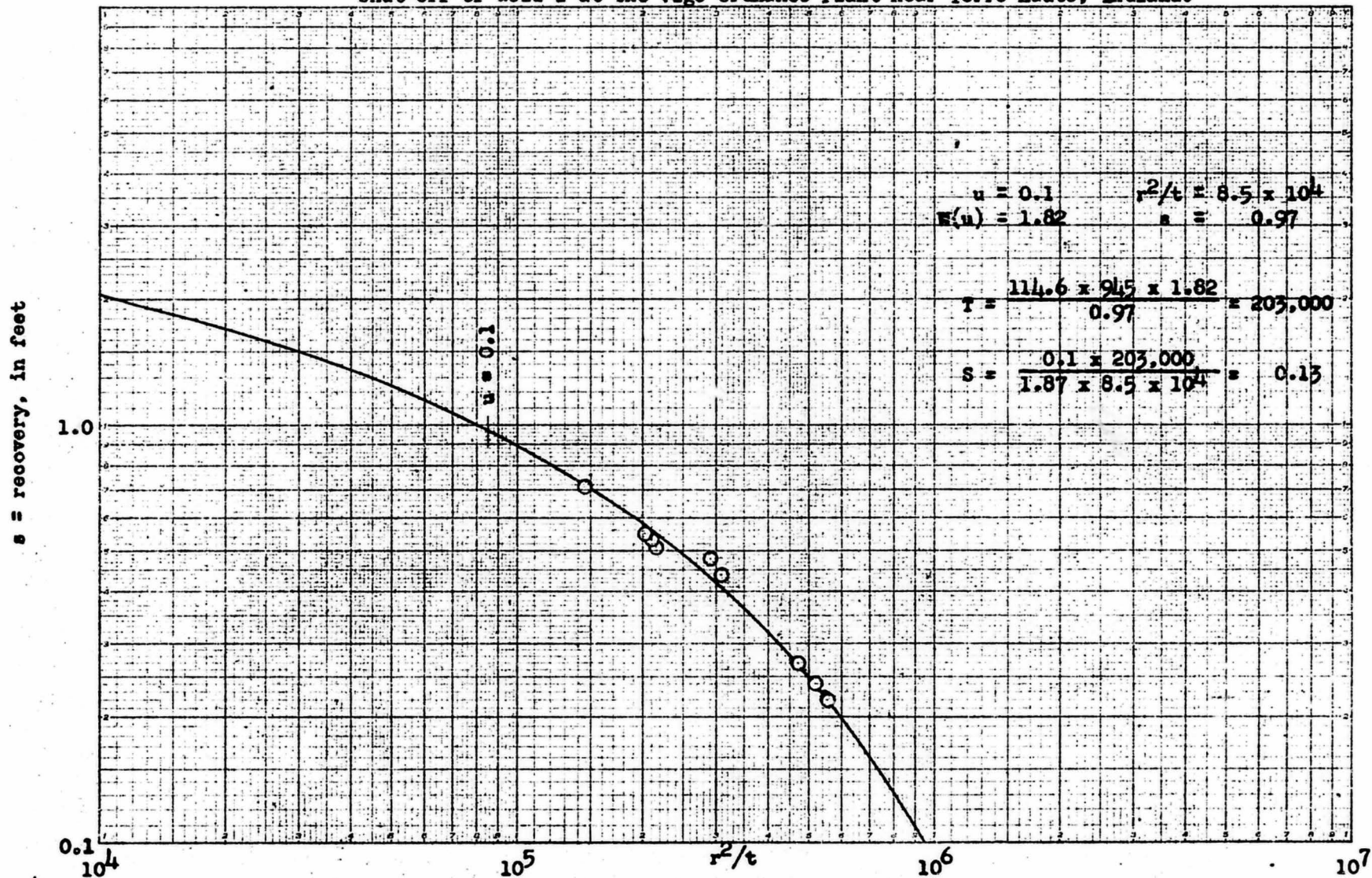
Fig. 16 -- Logarithmic graph of the recovery of water level in observation well P 3,2 after the shut-off of well 1 at the Vigo Ordnance Plant near Terre Haute, Indiana.
