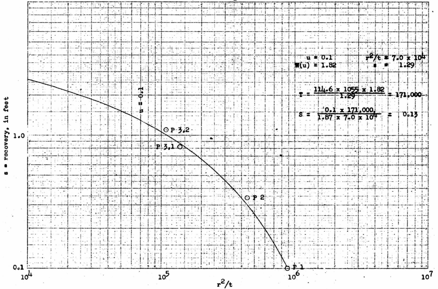
Fig. 17 -- Logarithmic graph of the recovery of water level in a profile line of observation wells after the shut-off of well 3 at the Vigo Ordnance Plant near Terre Haute, Indiana.
