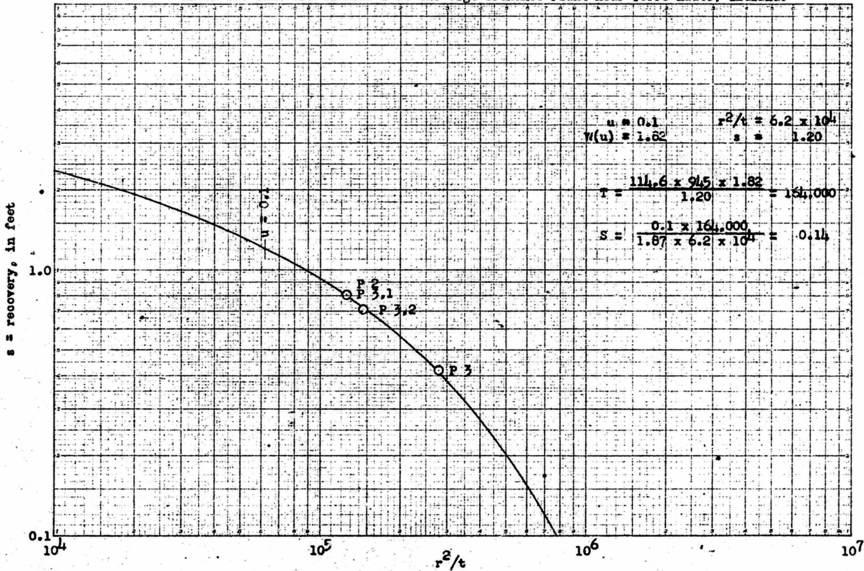
Fig. 18 -- Logarithmic graph of the recovery of water level in a profile line of observation wells after the shut-off of well 1 at the Vigo Ordnance Plant near Terre Haute, Indiana.
