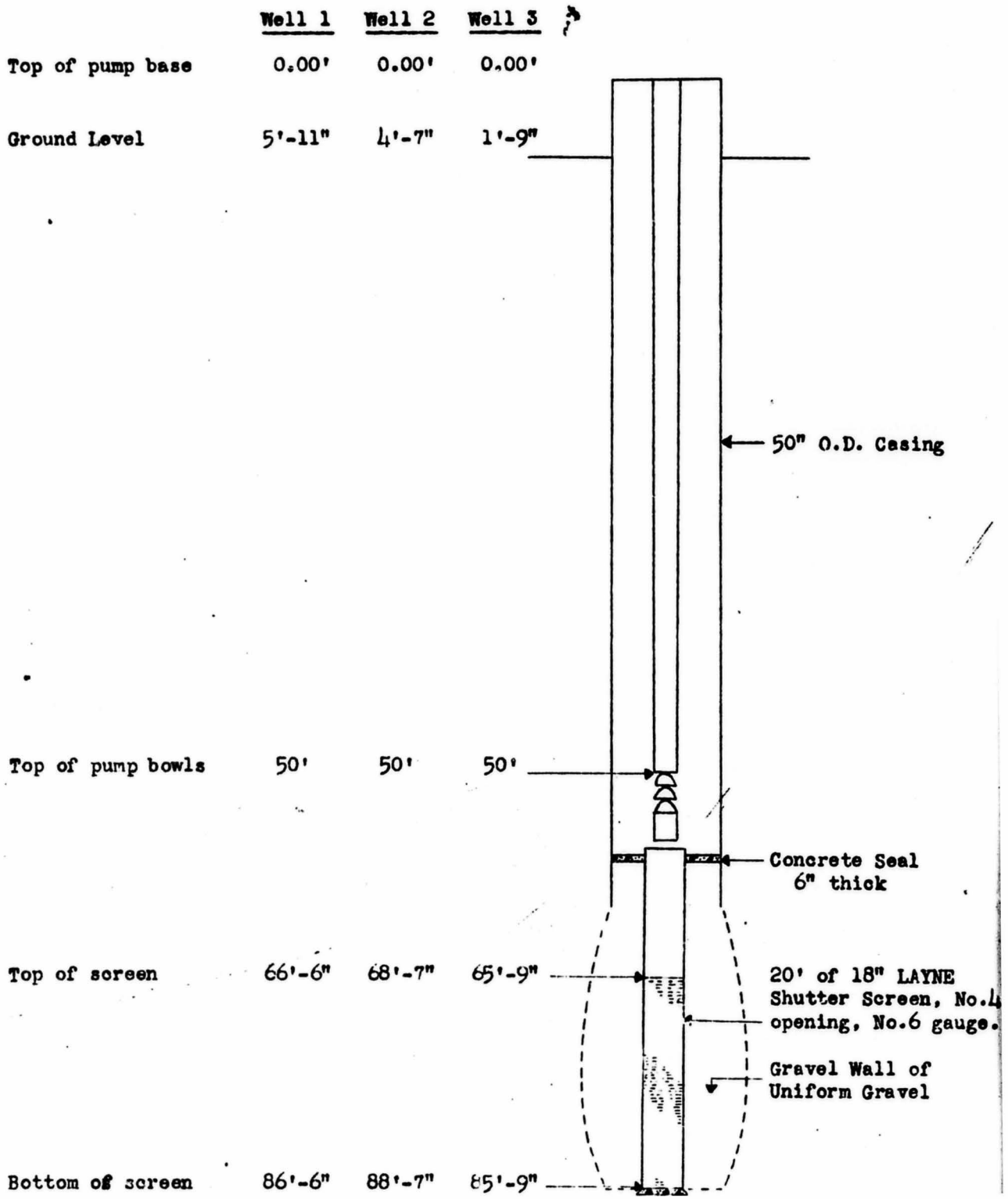
Fig. 19. Diagram showing construction of supply wells 1, 2, and 3 of the Vigo Ordnance Plant near Terre Haute, Indiana.
