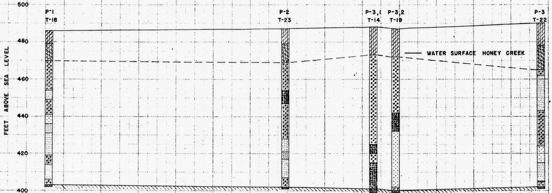
FIG. 3 - GENERALIZED CROSS-SECTION SHOWING SUCCESSION OF GLACIAL DEPOSITS THROUGH THE WELL FIELD OF THE VIGO ORDNANCE PLANT NEAR TERRE HAUTE, IND.
