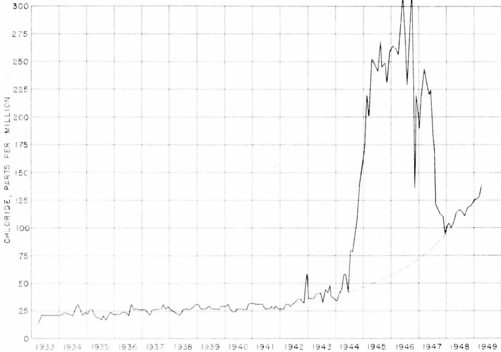
CHLORIDE CONTENT OF WATER FROM WELL 5/12-1161 IN THE ALAMITOS GAP, 1933-49
