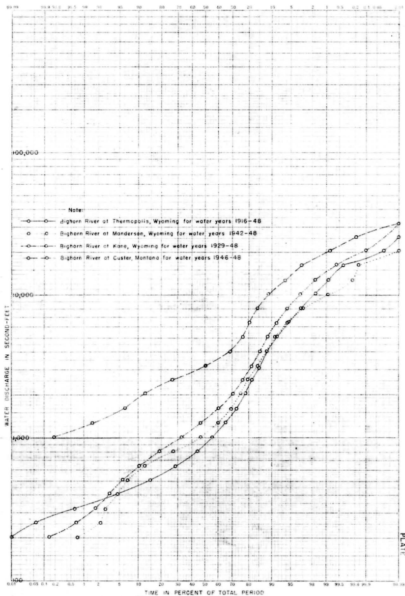
FLOW DEFICIENCY CURVES BIGHORN RIVER, WYOMING AND MONTANA
