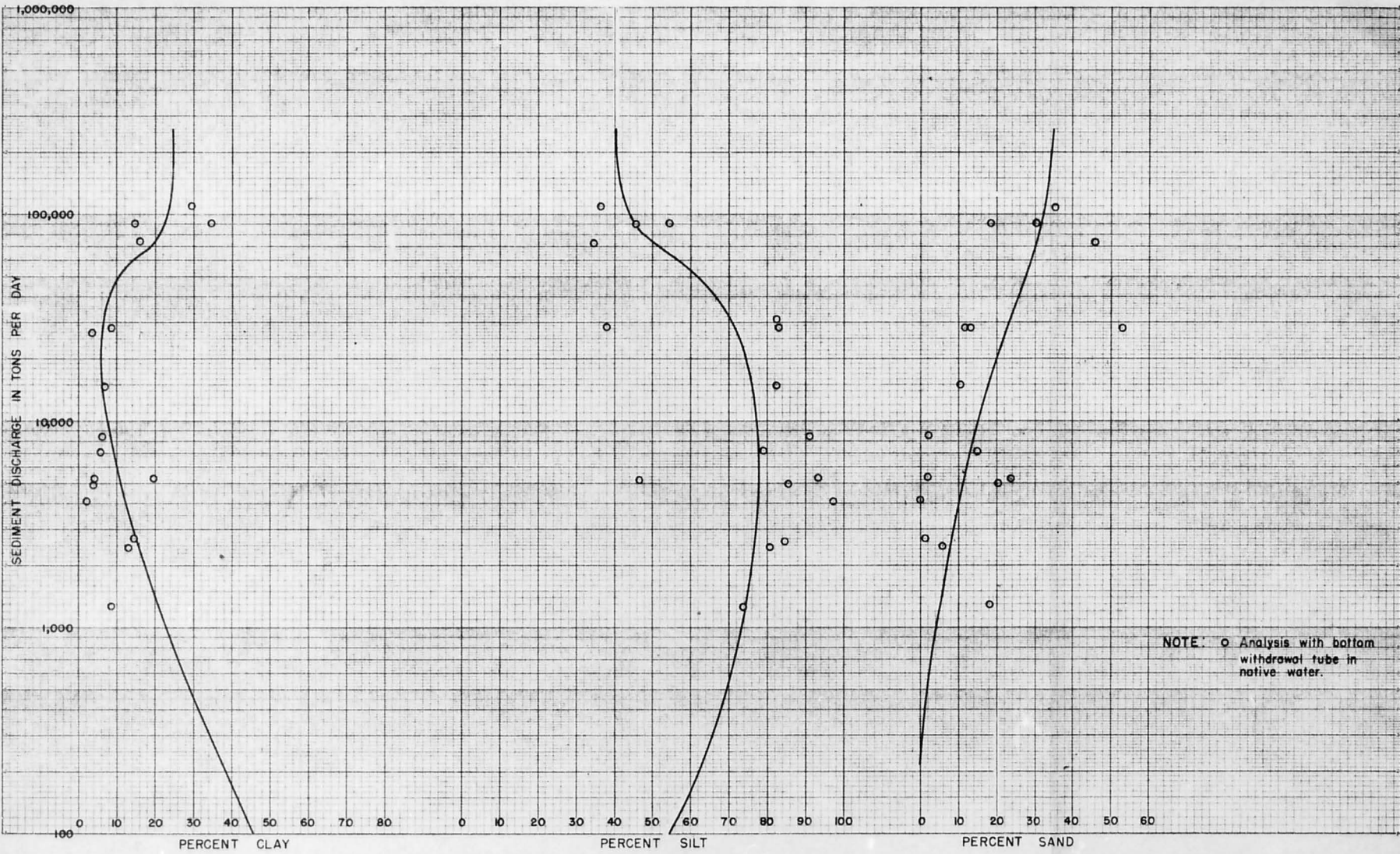
DISTRIBUTION OF SAND, SILT, AND CLAY WITH SUSPENDED SEDIMENT DISCHARGE, BIGHORN RIVER, THERMOPOLIS, WYOMING
