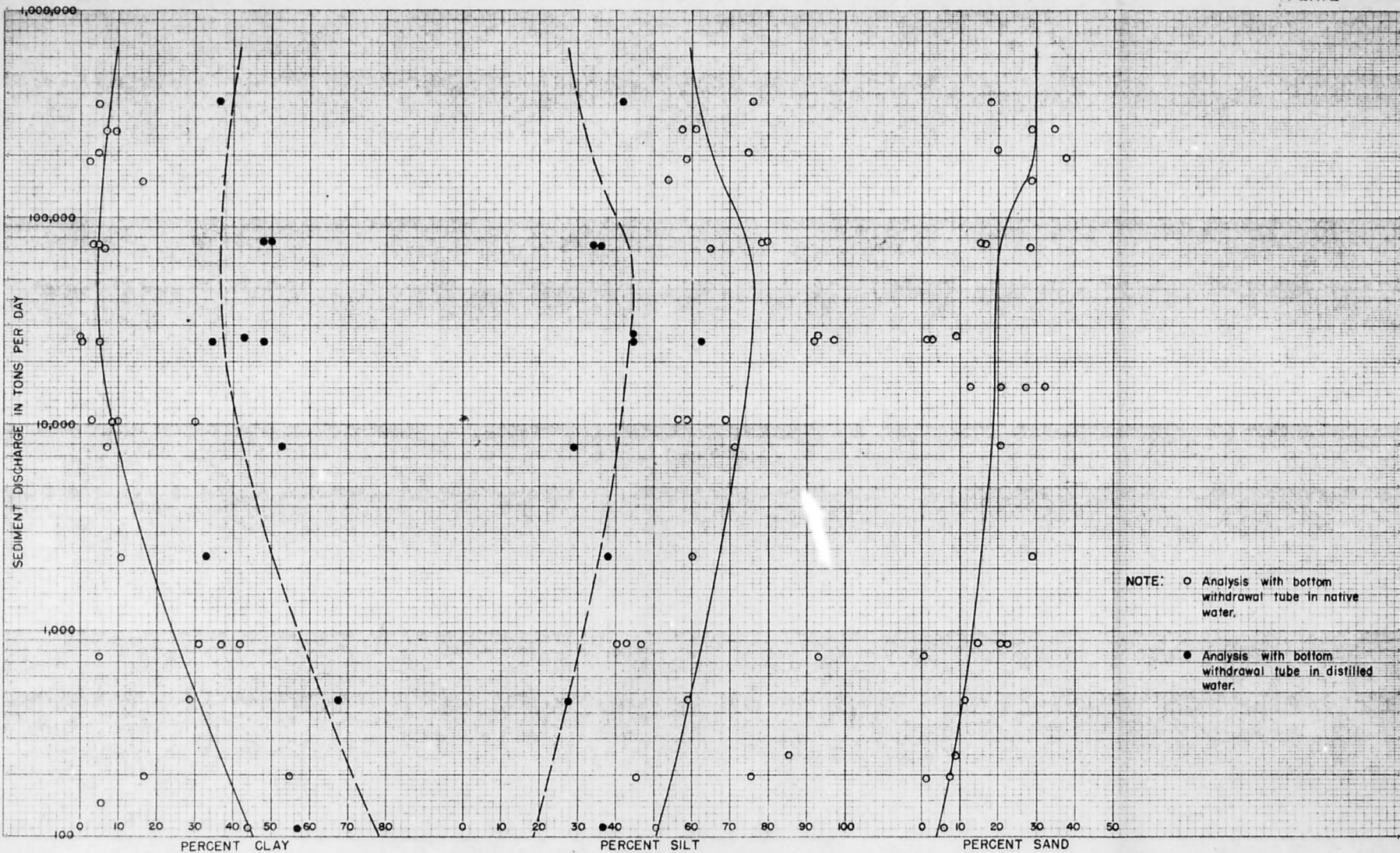
DISTRIBUTION OF SAND, SILT, AND CLAY WITH SUSPENDED SEDIMENT DISCHARGE, BIGHORN RIVER, MANDERSON, WYOMING
