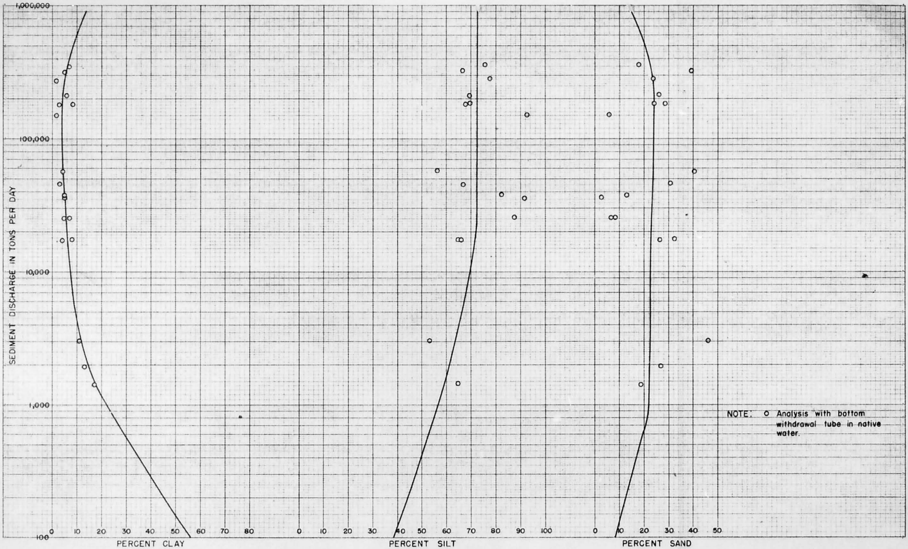
DISTRIBUTION OF SAND, SILT, AND CLAY WITH SUSPENDED SEDIMENT DISCHARGE, BIGHORN RIVER, KANE, WYOMING
