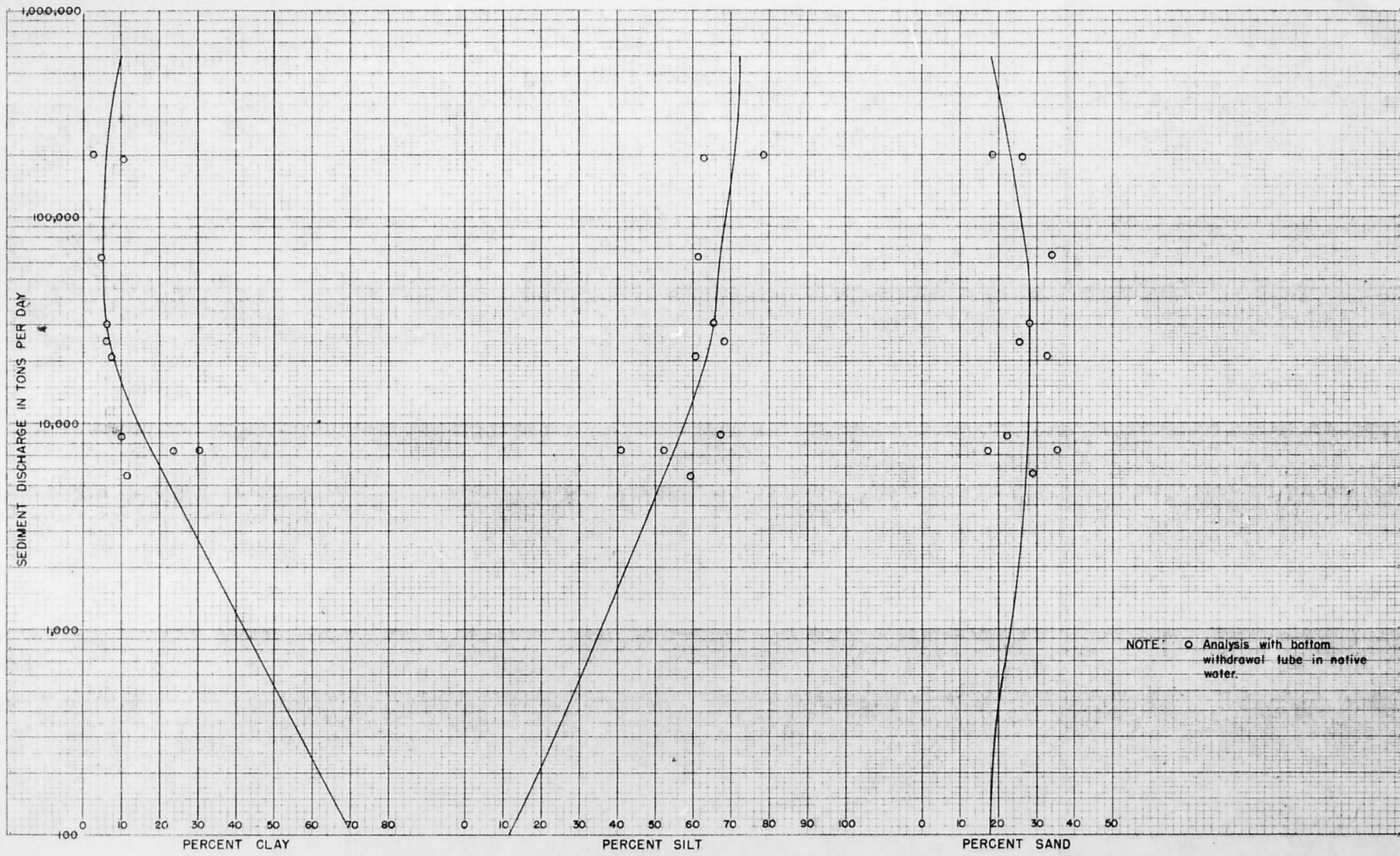
DISTRIBUTION OF SAND, SILT, AND CLAY WITH SUSPENDED SEDIMENT DISCHARGE, BIGHORN RIVER, CUSTER, WYOMING
