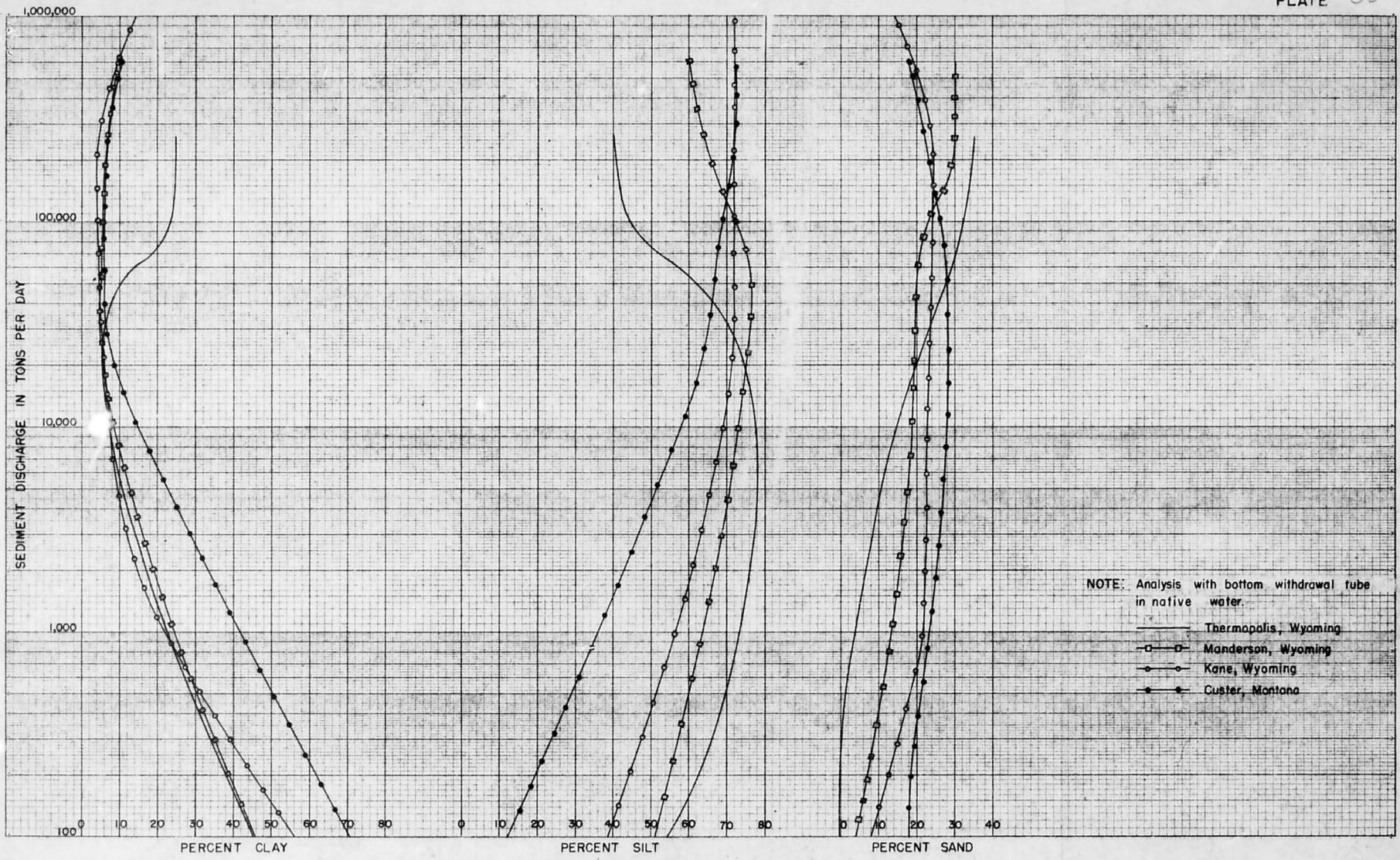
DISTRIBUTION OF SAND, SILT, AND CLAY WITH SUSPENDED SEDIMENT DISCHARGE, BIGHORN RIVER
