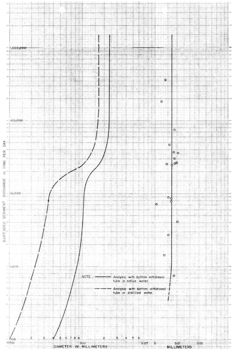
DISTRIBUTION OF MEDIAN PARTICLE SIZE WITH SUSPENDED SEDIMENT DISCHARGE BIGHORN RIVER, WYOMING AND MONTANA
