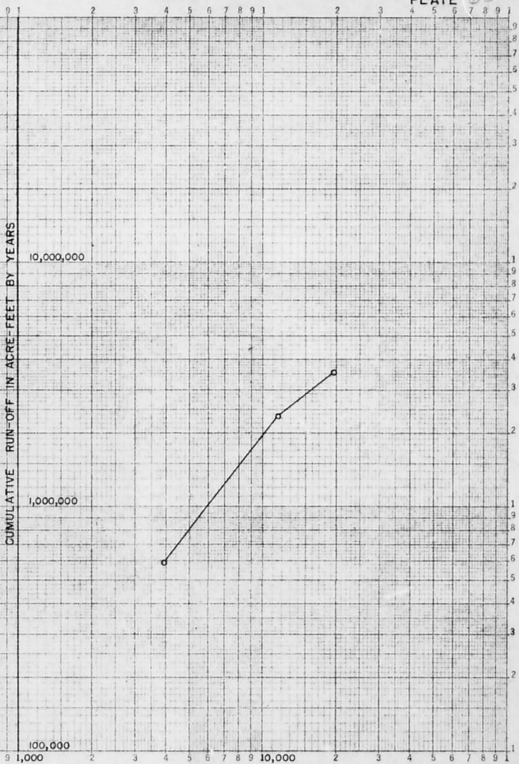
CUMULATIVE WATER AND SUSPENDED SEDIMENT DISCHARGE, APRIL 1946-SEPTEMBER 1948, MANDERSON, WYOMING
