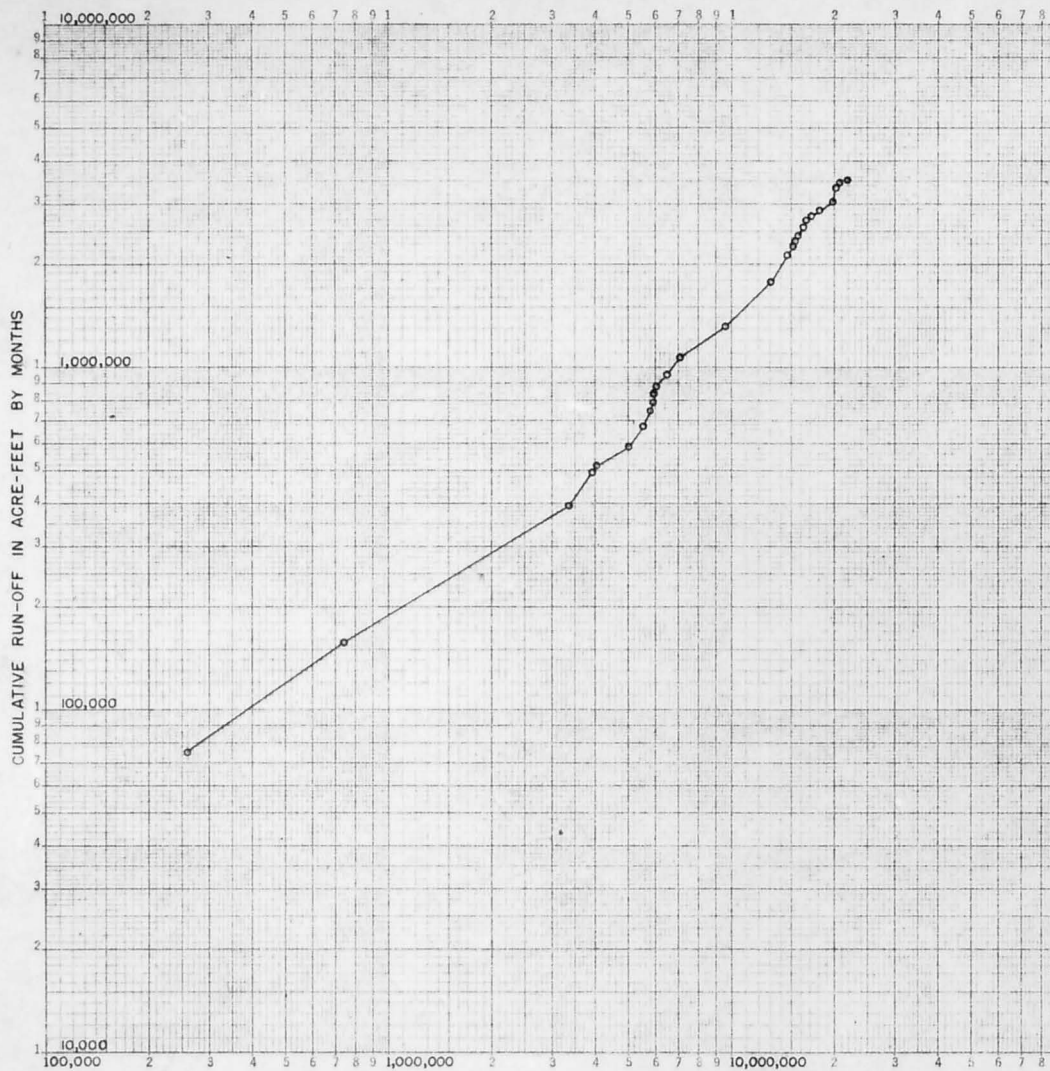
CUMULATIVE WATER AND SUSPENDED SEDIMENT DISCHARGE, APRIL 1946-SEPTEMBER 1948, MANDERSON, WYOMING
