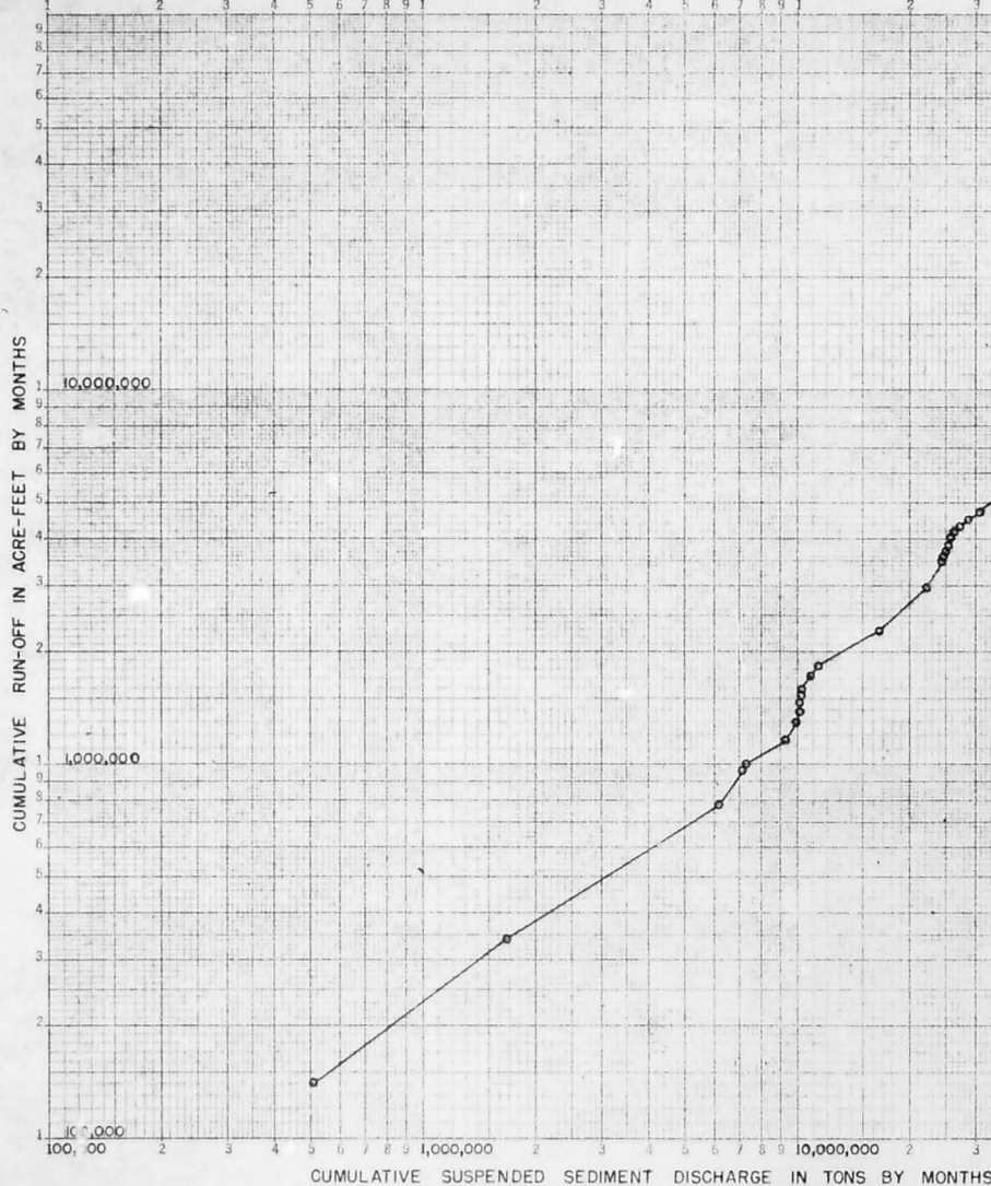
CUMULATIVE WATER AND SUSPENDED SEDIMENT DISCHARGE, APRIL 1946-SEPTEMBER 1948, KANE, WYOMING
