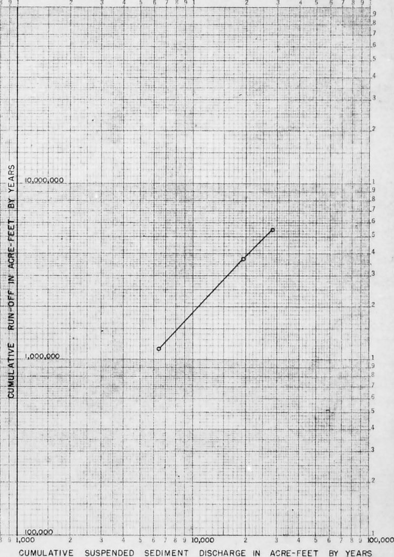
CUMULATIVE WATER AND SUSPENDED SEDIMENT DISCHARGE, APRIL 1946-SEPTEMBER 1948, KANE, WYOMING
