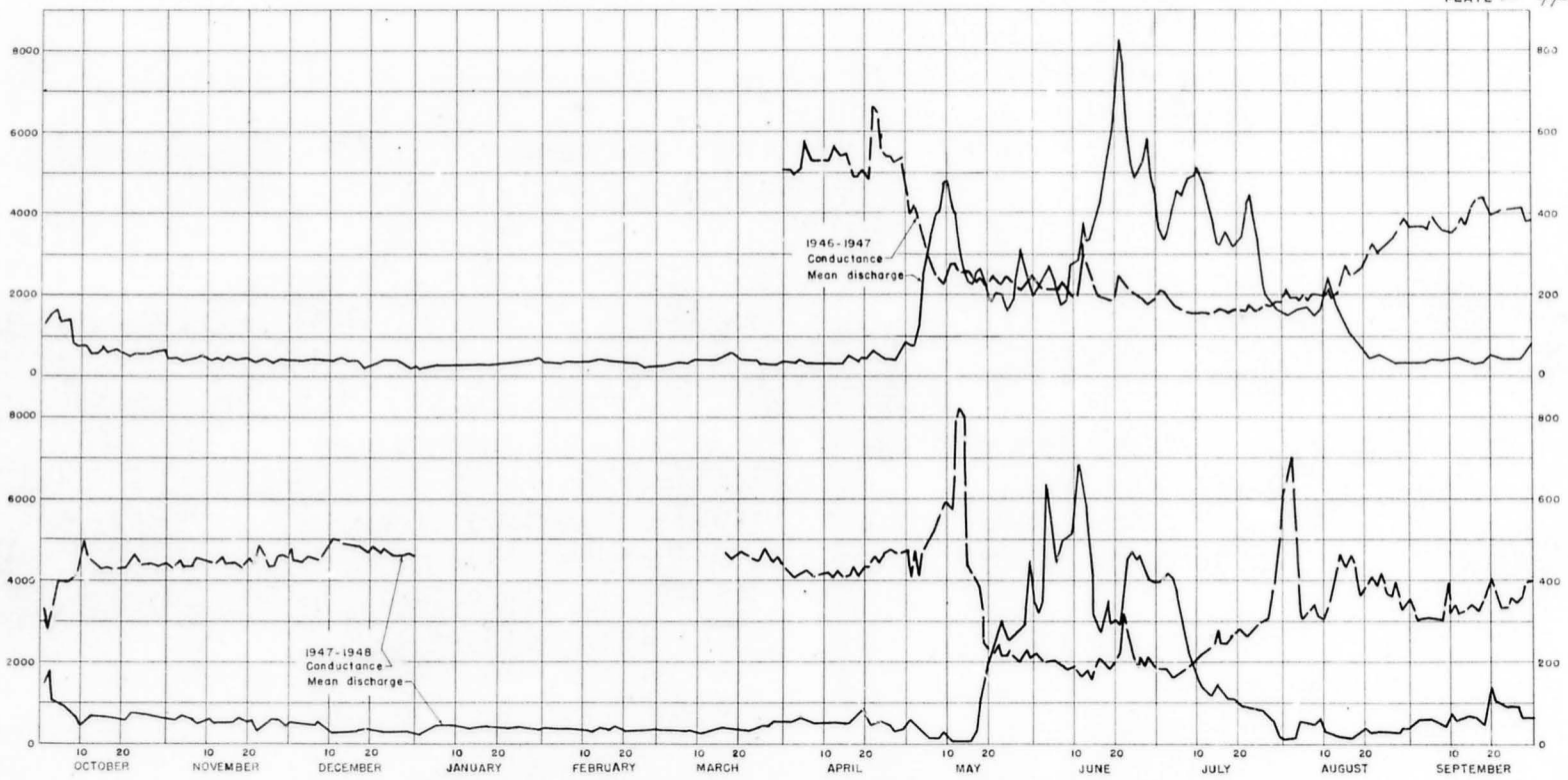
DAILY SPECIFIC CONDUCTANCE AND MEAN DAILY DISCHARGE WIND RIVER, RIVERTON, WYOMING
