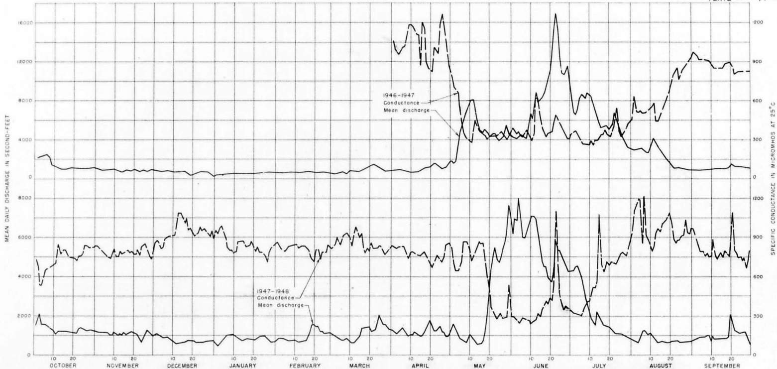
DAILY SPECIFIC CONDUCTANCE AND MEAN DAILY DISCHARGE BIGHORN RIVER, THERMOPOLIS, WYOMING.
