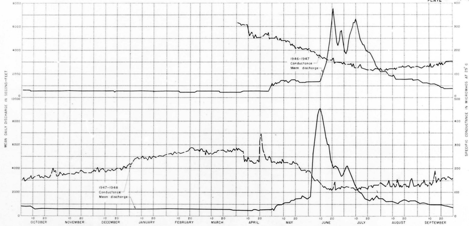
DAILY SPECIFIC CONDUCTANCE AND MEAN DAILY DISCHARGE SHOSHONE RIVER BELOW BUFFALO BILL RESERVOIR, CODY, WYOMING.
