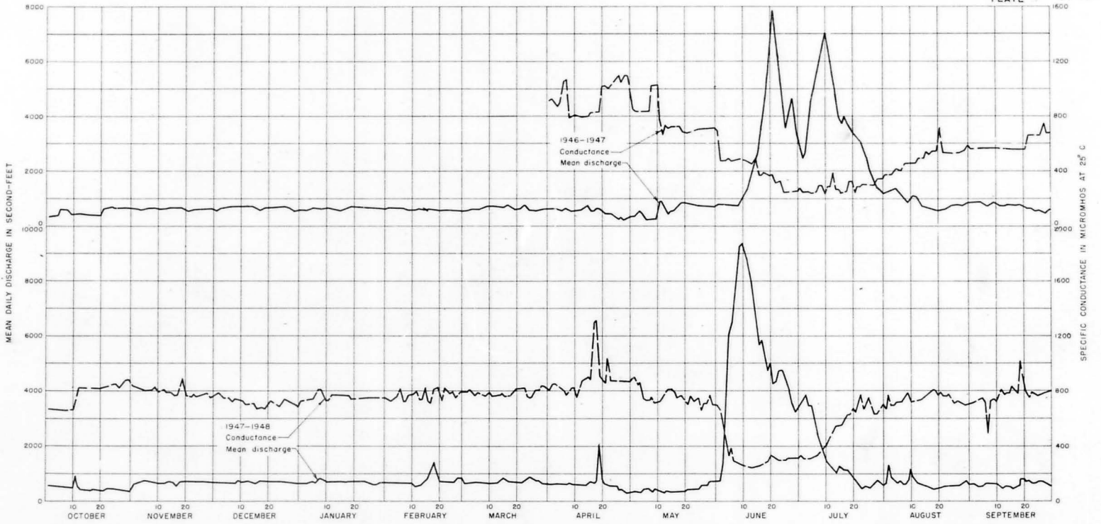
DAILY SPECIFIC CONDUCTANCE AND MEAN DAILY DISCHARGE SHOSHONE RIVER, BYRON, WYOMING
