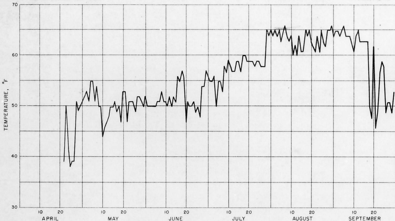
DAILY WATER TEMPERATURES OF WIND RIVER WATERS NEAR DUBOIS, WYOMING, APRIL-SEPTEMBER 1947.
