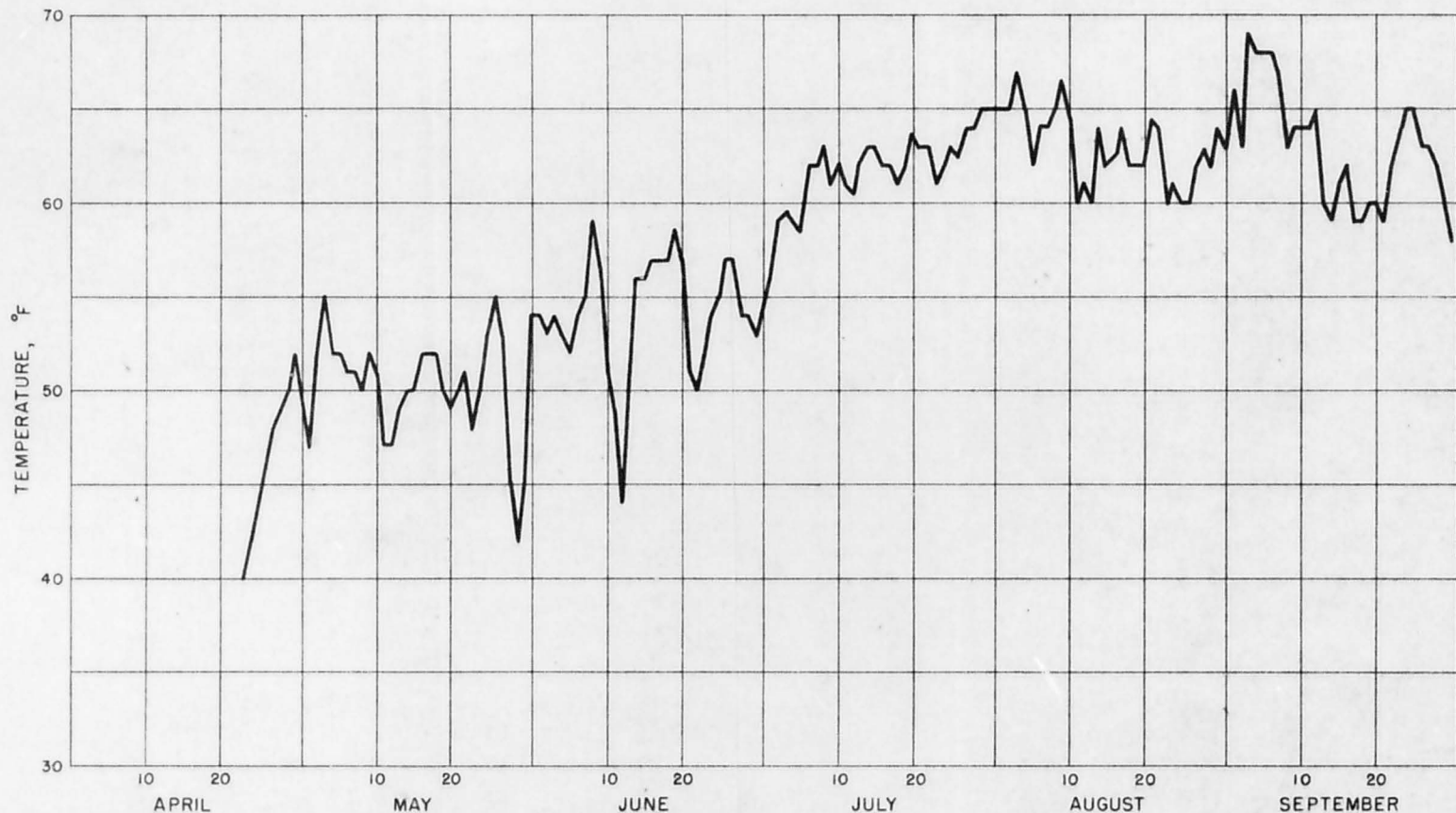
DAILY WATER TEMPERATURES OF WIND RIVER WATERS NEAR RIVERTON, WYOMING, APRIL-SEPTEMBER 1947.
