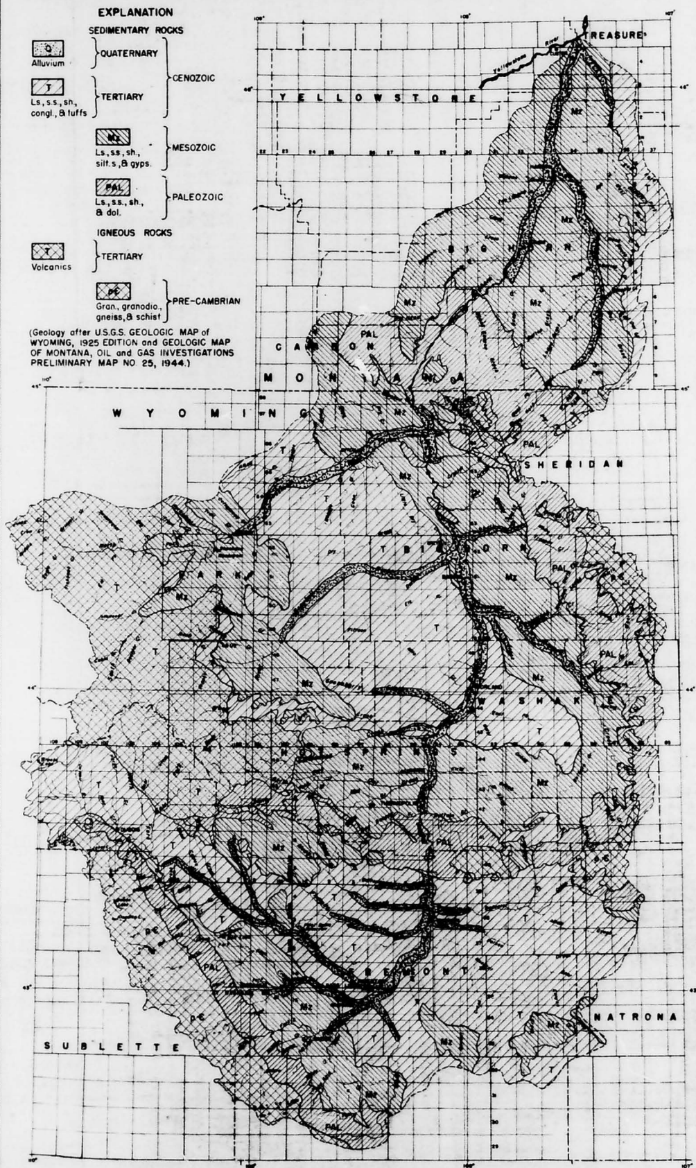
GEOLOGIC MAP OF BIGHORN RIVER DRAINAGE BASIN, WYOMING & MONTANA
